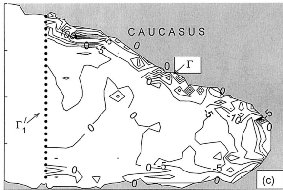
FIG. 10. Vertical velocity (in 10^{-4} \text{ cm s}^{-1} ) at 20 m deep: (a) exact data, (b) reconstructed field from deposition A sampling with a white noise ( \eta_1 = 0.3 ), and (c) error ( w_{\text{res}} ). The positive values indicate upwelling.
