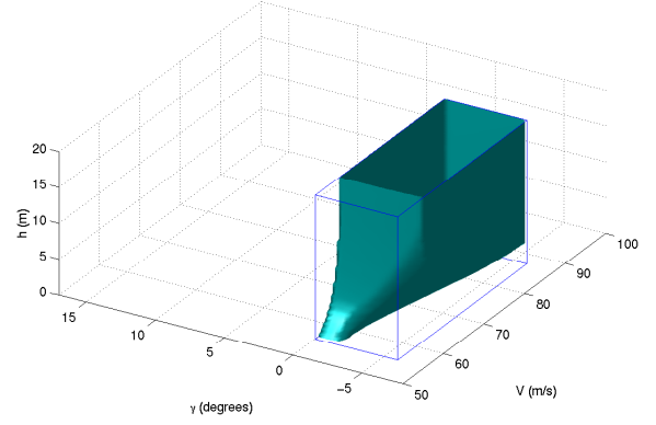
Figure 3: Safe region \mathcal{W}_F ; the outer box is (\mathcal{W}_F)_0 .
