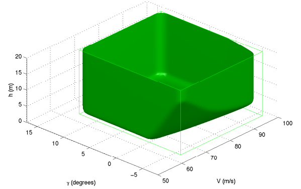
Figure 4: Safe region \mathcal{W}_T ; the outer box is (\mathcal{W}_T)_0 .
