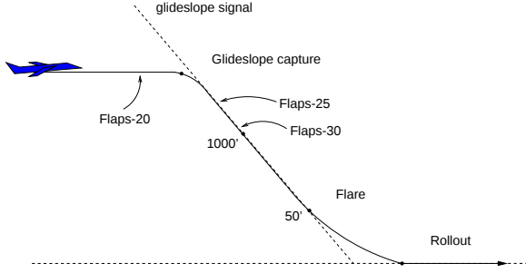
Figure 1: Typical landing scenario.
