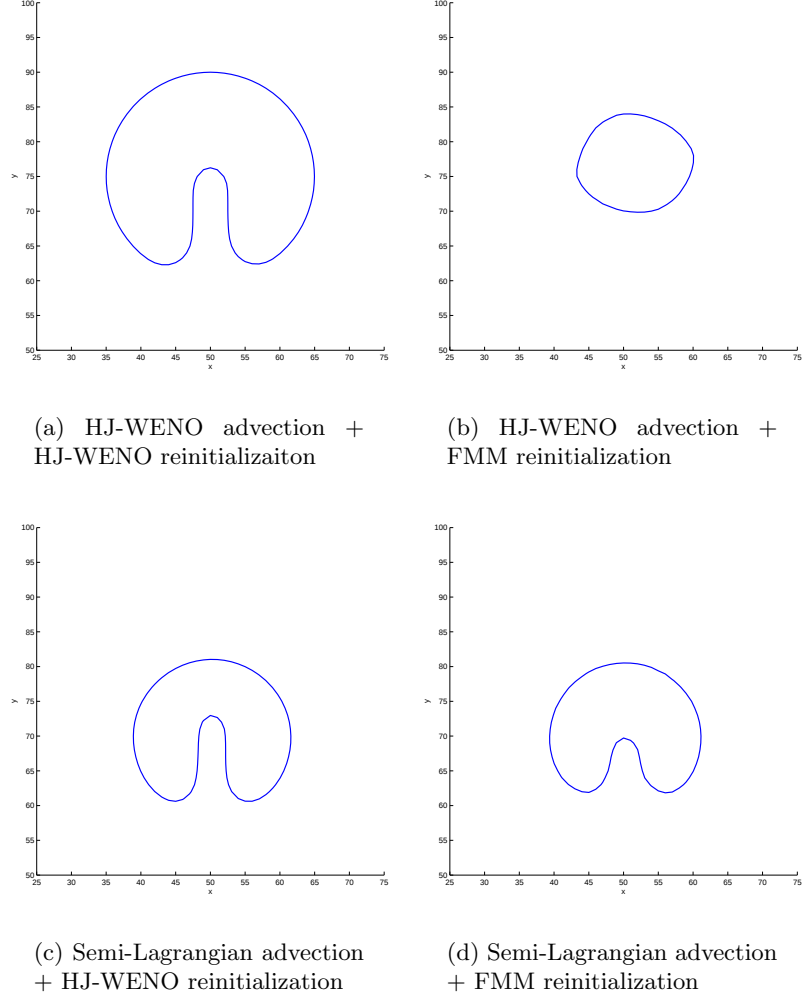
Figure 1: Level set only method. Comparison of various advection and reinitialization algorithms after one revolution on a 100 \times 100 grid cell computational domain.
