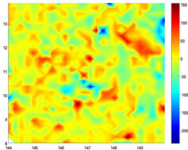
Figure 12. Difference between acoustic coverages computed using nominal and true depth for an area in the western Pacific ocean. Color represents coverage area in \text{km}^2 .
