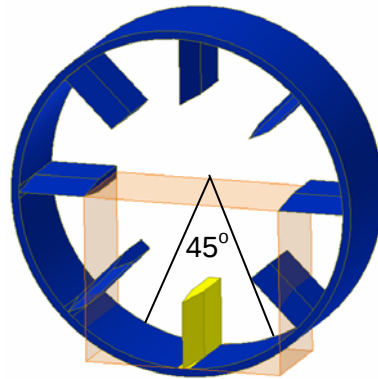
Figure 2 A single strut in a 12.7\text{ cm} \times 15.24\text{ cm} (5" x 6") rectangular flow path with a 25.4\text{ cm} (10") round combustor with eight-strut injection overly.
