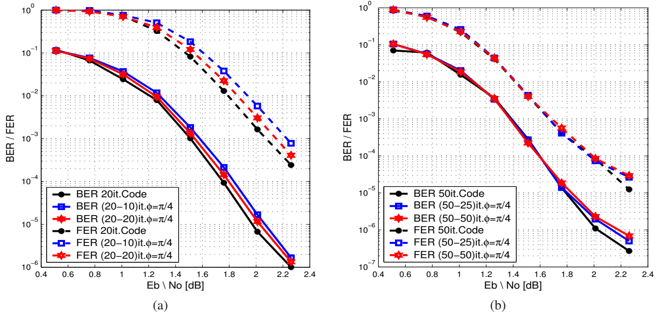
Fig. 4. IRCS BER/FER performance with a maximum of (a) 20 and (b) 50 LDPC iterations.
