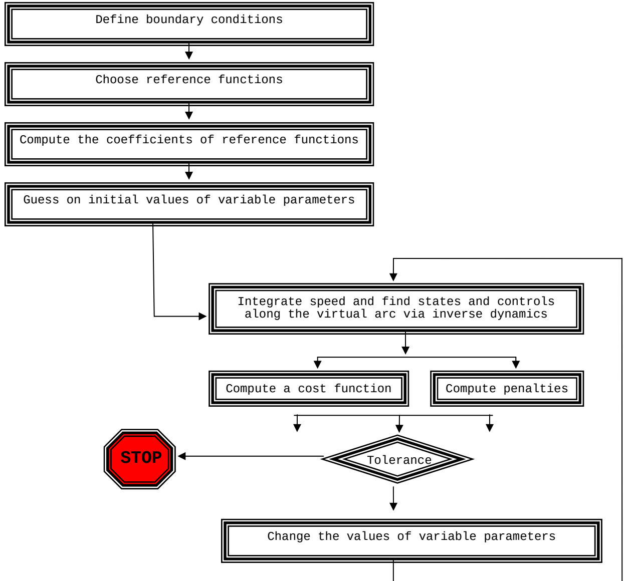
Figure 10. General Block-Scheme
