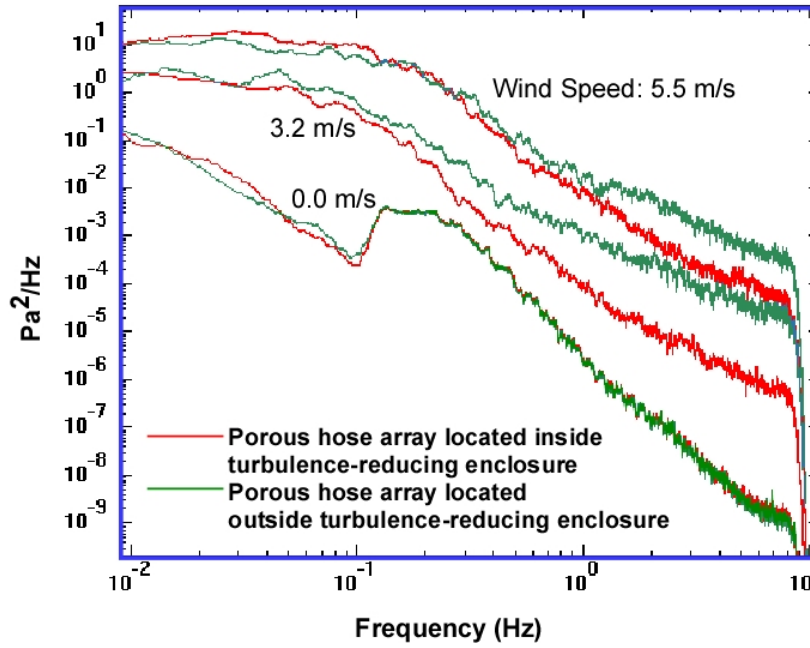
Figure 34. Power spectral density of background noise recorded using a conventional porous hose pipe array system located inside Version 1 of the enclosure with 1.6-m high walls (red curves) compared with the power spectral density of background noise recorded simultaneously on an identical pipe array system located outside the enclosure (green curves) for wind speeds (at a height of 2.0 m) of 0.0, 3.2 and 5.5 m/s.
