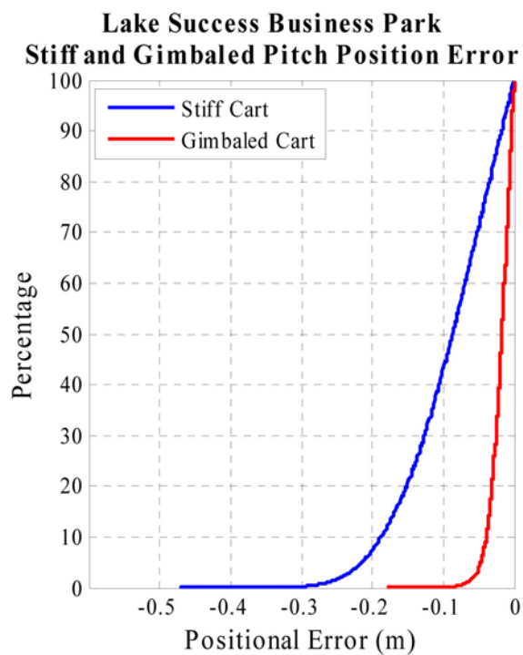
Figure 41. Cumulative distribution plots of positional errors associated with the pitch tilt of the EM systems for standard EM61 stiff and gimbal system.
