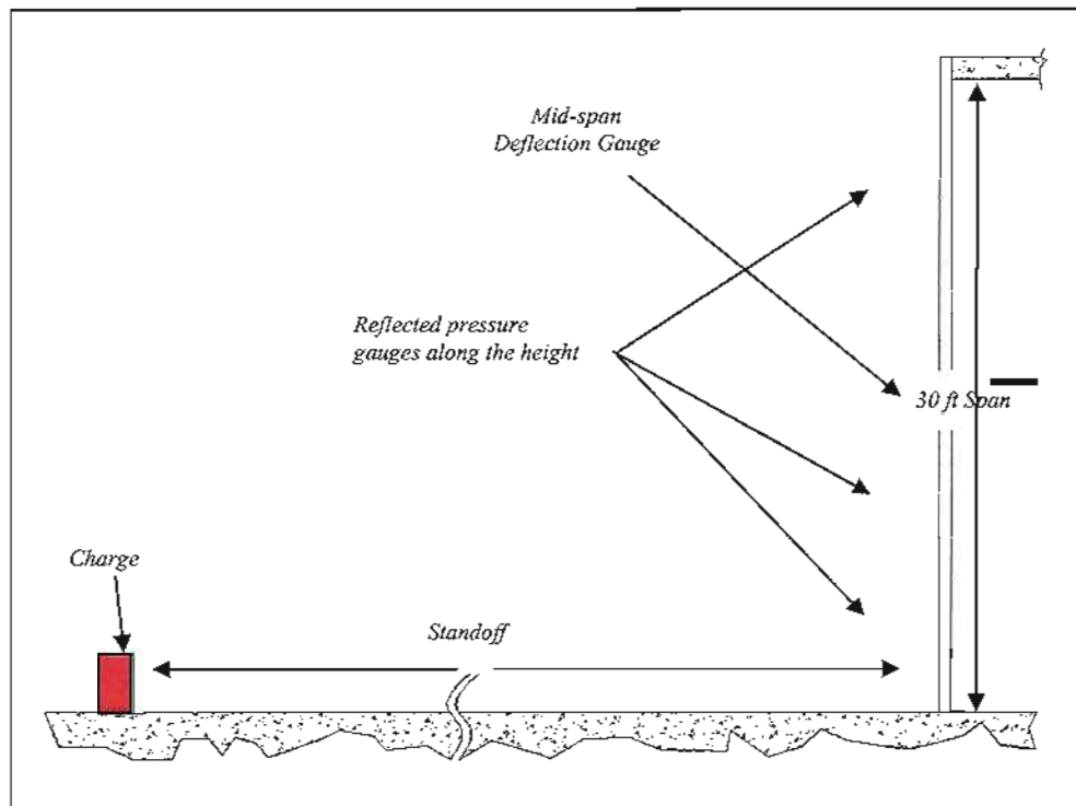
Figure 7 Test Setup
