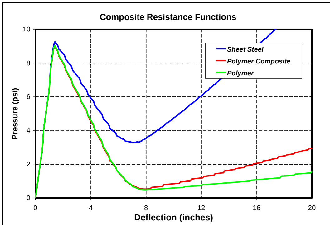
Figure 9 Combined Sheet and Arching Resistance Function
