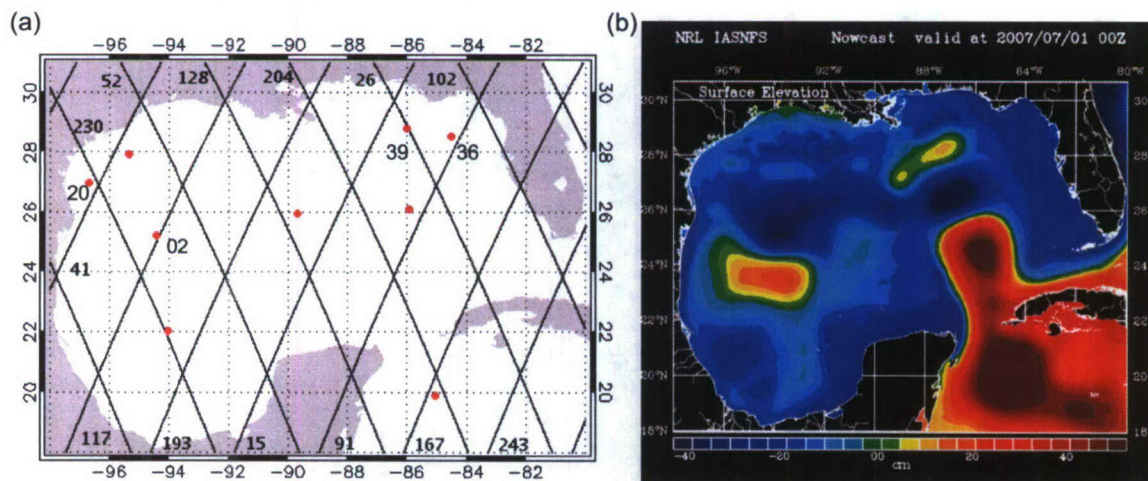
Fig. 1. (a) Map of the study area showing the ground-track lines of Jason-1. The red circles denote the locations of NDBC buoys located in the GOM. (b) Corresponding segment of the IASNFS NCOM model output of SSH used in the comparison study.
