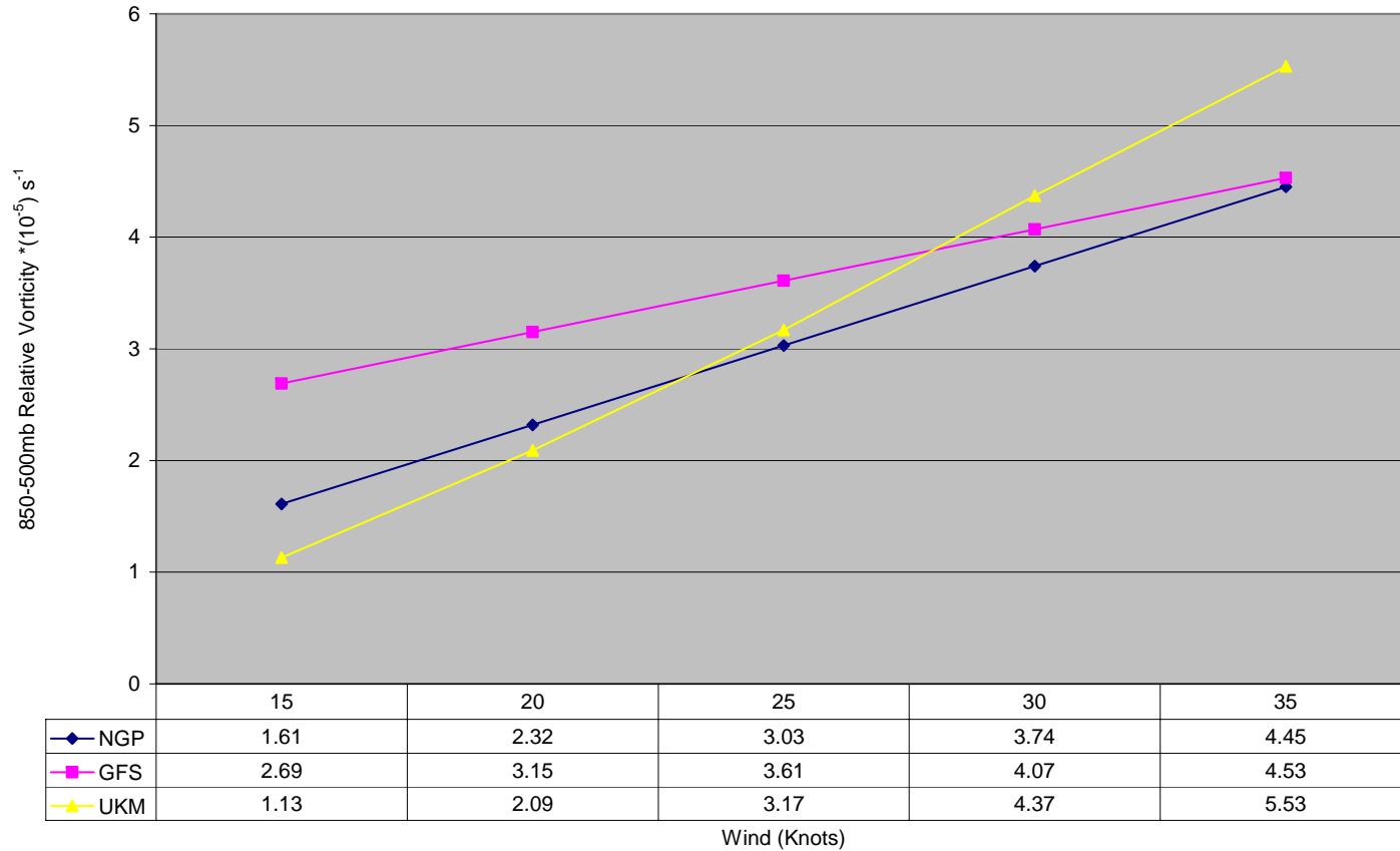
Figure 3 Smoothed Lower Tercile Values (LTVs) for 850 - 500 mb relative vorticity ( 10^{-5} \text{ s}^{-1} ) corresponding to the CARQ intensities (kt) for the NOGAPS (diamond symbols), GFS (square symbols), and the UKMO (triangle symbols).
