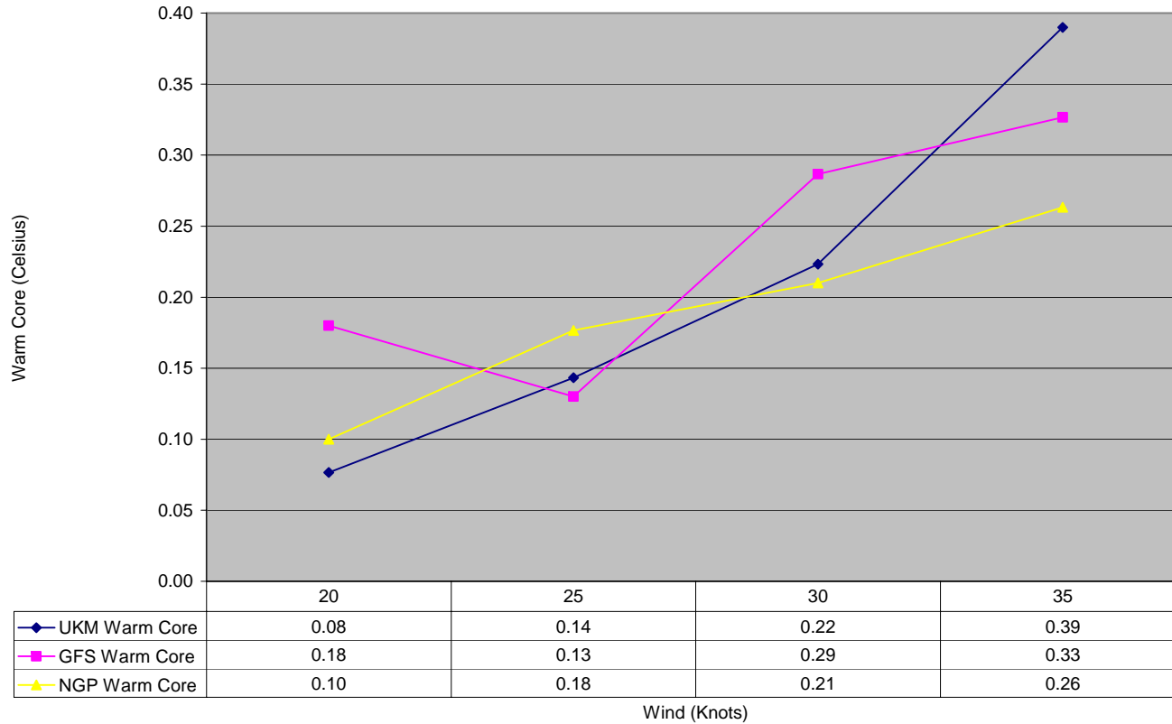
Figure D-10. Comparison of all models LTV for 700 - 500 mb warm core at 20, 25, 30, and 35 kt using statistical method
