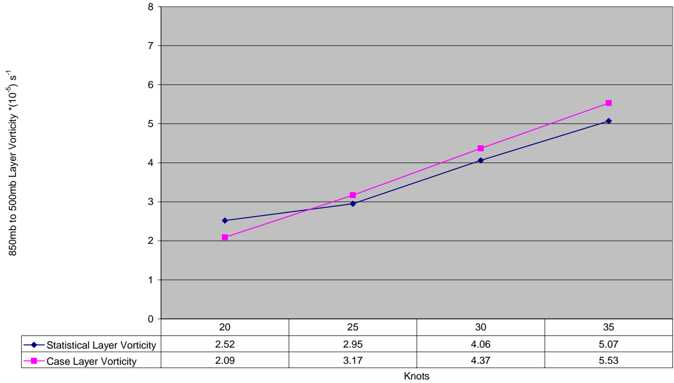
Comparison of Methods of Layer Vorticity Lower Tercile Values (UKM)
