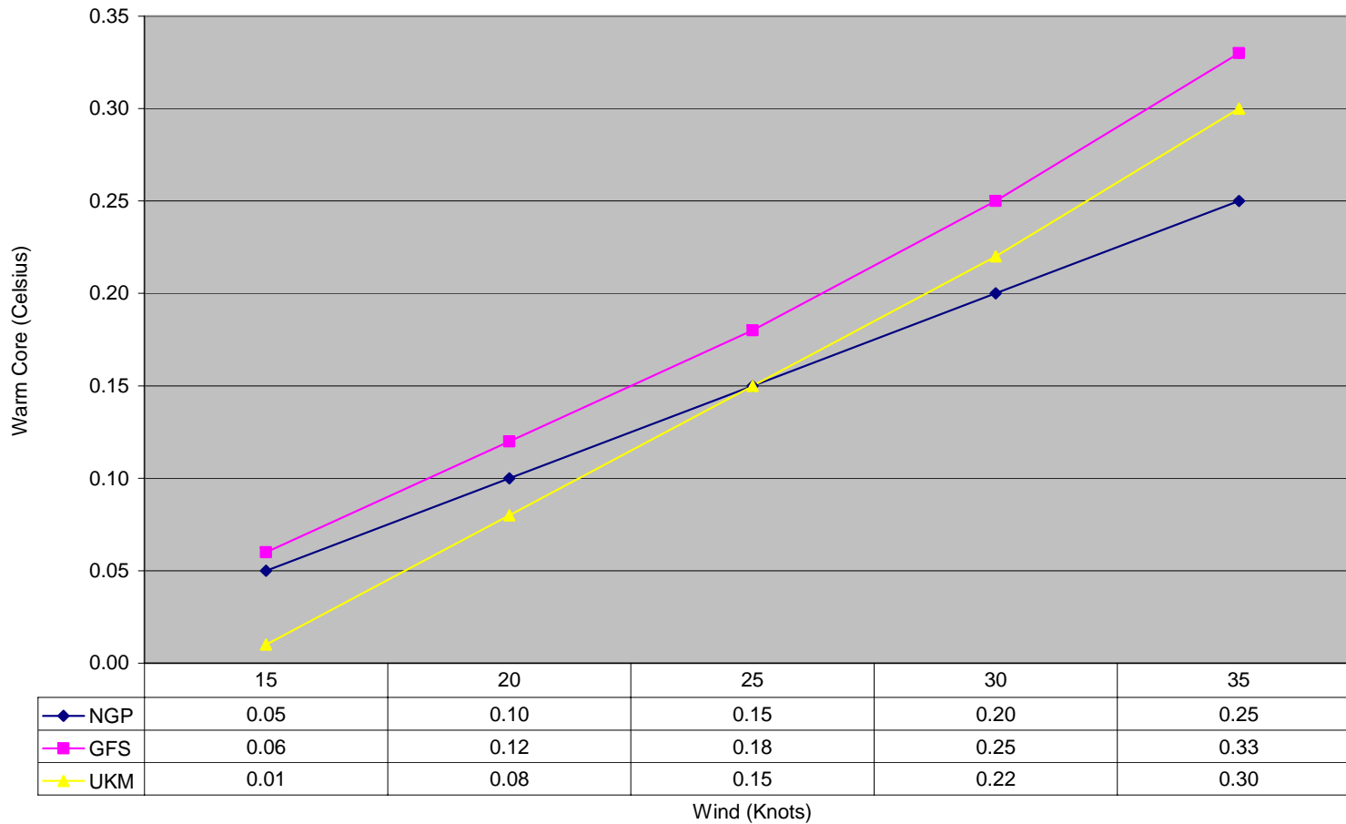
Figure 4 As in Figure 3, except for 700 - 500 mb warm core (°C).
