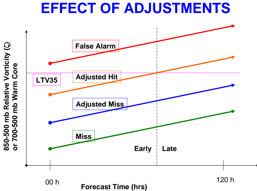
Figure 8 Schematic of the forecast evaluations for unadjusted and adjusted initial conditions that result in false alarms (exceeds LTV_{35} from the beginning) or misses (does not exceed LTV_{35} during the forecast interval) versus adjusted initial conditions that may result in a hit or a miss. For both the unadjusted and the adjusted forecasts, the forecast time may be either early or late relative to the verification time (CARQ intensity equal to 35 kt).
