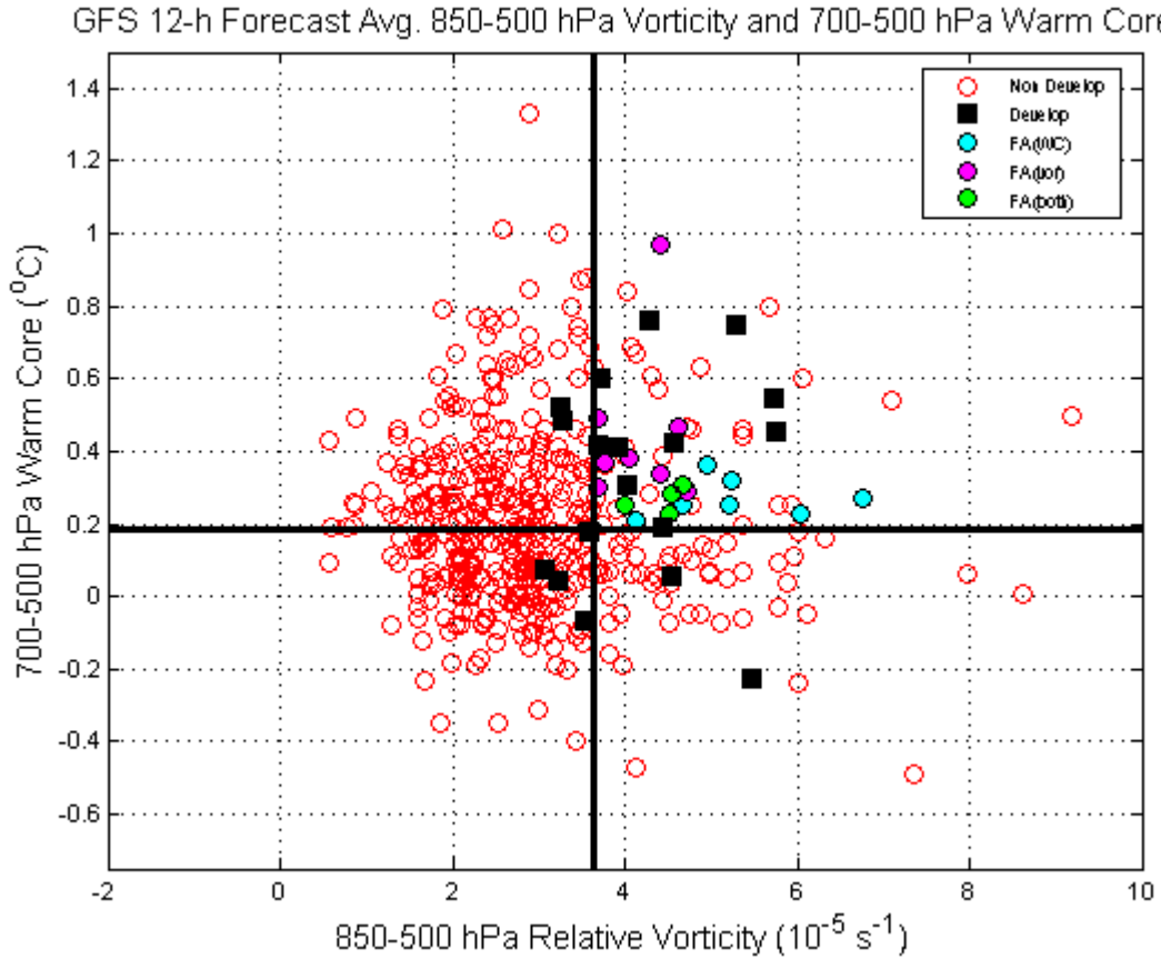
Figure 5 Scatterplot of 850 - 500 mb average relative vorticity and 700 - 500 mb warm core for the 12 h GFS vortices in the VORTRACK data base of 2005 Atlantic season tropical cyclones from Cowan (2006; Figure 4). The dark lines are the threshold values for these two variables that if surpassed would indicate tropical cyclone formation. The symbols (see inset) represent non-developers (open circles), developers (squares), and three kinds of False Alarms (filled circles).
