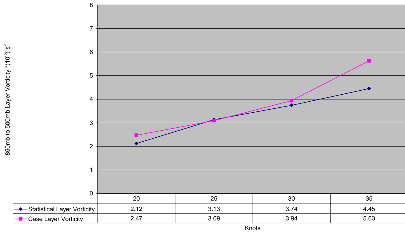
Figure D-1. NOGAPS LTV for case and statistical methods of calculating 850 - 500 mb relative vorticity for 20, 25, 30, and 35 kt.
