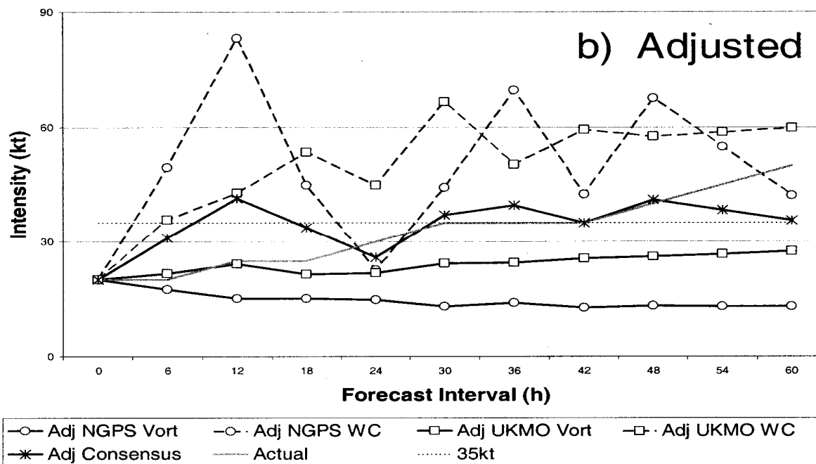
Figure 10 Intensity forecasts converted from the (a) unadjusted and (b) adjusted NOGAPS 850 - 500 mb relative vorticity and 700 - 500 mb warm core forecasts (see inset) from 0000 UTC 8 June 2005 for Tropical Depression Arlene. The consensus of these intensity forecasts and the verifying CARQ intensities are also indicated.
