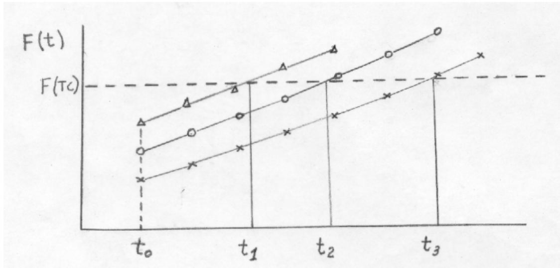
Figure 1 Time evolution schematic. Schematic of the time evolution of three numerical model solutions F(t) beginning from time t_0 , and the times ( t_1, t_2, t_3 ) at which a threshold condition for tropical cyclone formation F(TC) is first met. The middle solution ( \circ symbols) with a formation time t_2 is considered to be the truth and the upper solution ( \Delta symbols) and lower solution ( \times symbols) begin from erroneous initial conditions and thus result in erroneous tropical cyclone formation times t_1 and t_3 , respectively.
