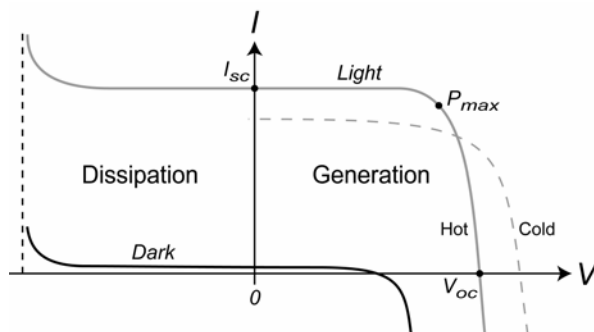
Figure 9: Current-voltage behavior of silicon photovoltaic cells with (light) and without (dark) incident radiation. Decreasing cell temperature lowers the short-circuit current, I_{sc} , and increases the open-circuit voltage, V_{oc} , leading to a net increase in output power.
