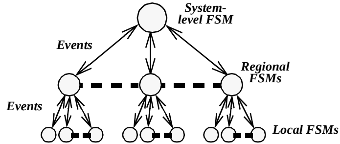
Figure 9: Network of communicating finite-state machines
