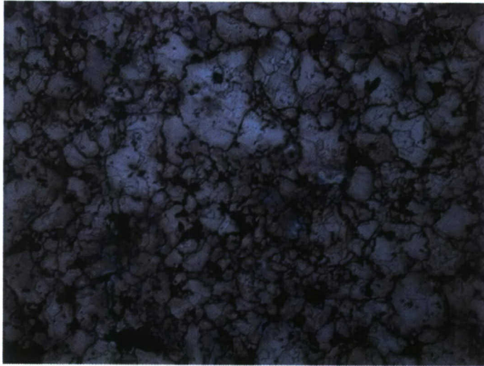
Figure 2.8: Optical microscopy image of a cold pressed Fe sample.
