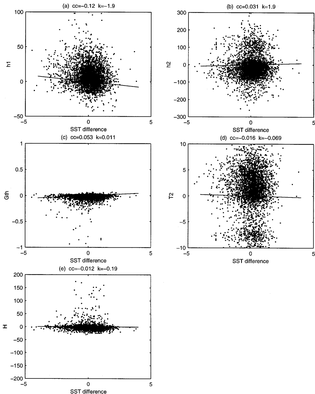
FIG. 7. Scatter diagrams of SST anomaly with various thermal parameter anomalies: (a) h'_1 , (b) h'_2 , (c) G'_{th} , (d) T'_{th} , and (e) H' .
