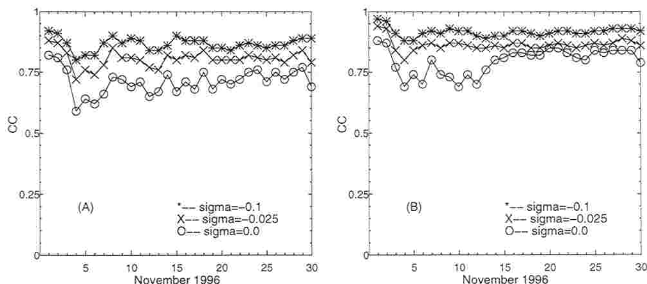
Figure 14. Correlation coefficient of the model currents at different \sigma levels under NSCAT and NCEP wind forcing for (a) u and (b) v components.
