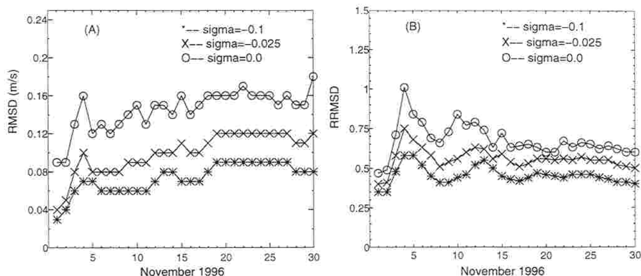
Figure 13. Temporally varying (a) rmsd and (b) rrmsd of the model currents at different \sigma levels under NSCAT and NCEP wind forcing.
