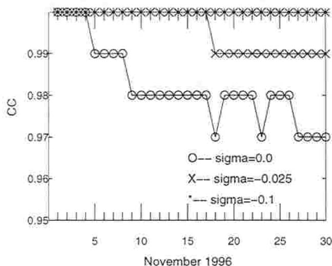
Figure 17. Correlation coefficient of model temperature.
