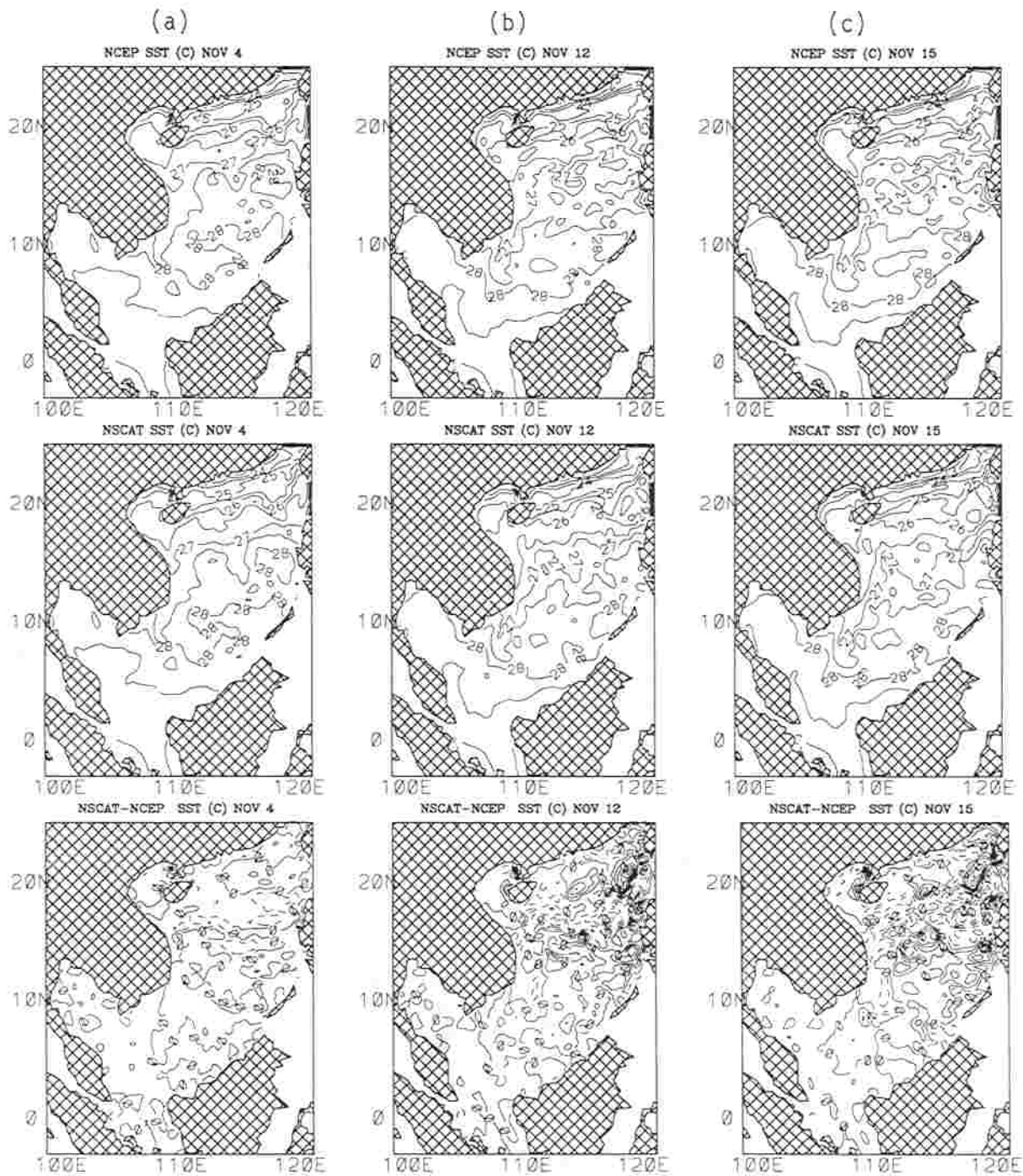
Figure 15. Same as Figure 12, except for the model temperature.
