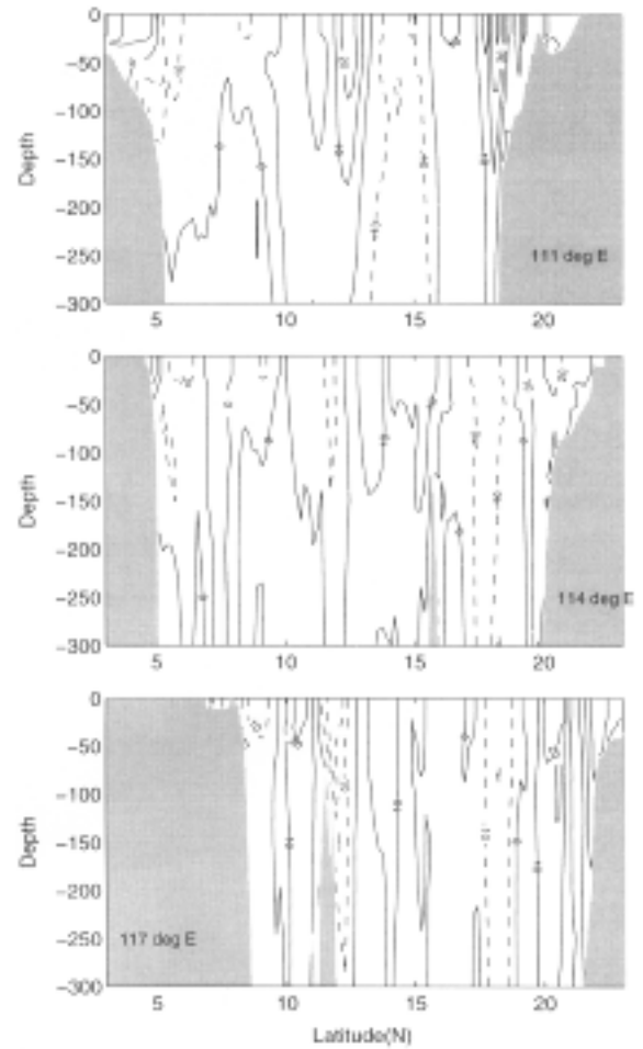
Fig. 15. CAOCS simulated mean velocity u -component in \text{cm s}^{-1} during 14–25 May 1995 at several latitudinal cross section: (a) 111°E, (b) 114°E, and (c) 117°E.
