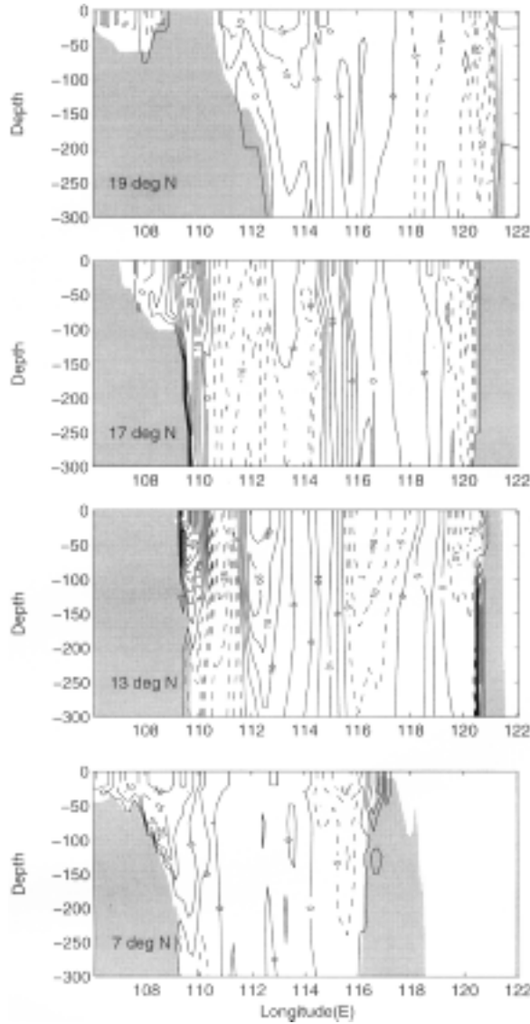
Fig. 14. CAOCS simulated mean velocity v -component in \text{cm s}^{-1} during 14–25 May 1995 at several zonal cross section: (a) 19°N, (b) 17°N, (c) 13°N, and (d) 7°N.
