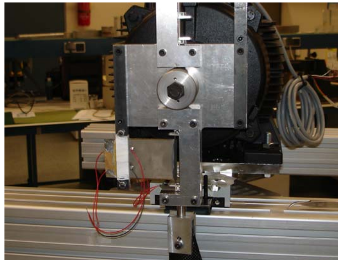
Figure 7: The smart support system realized.
