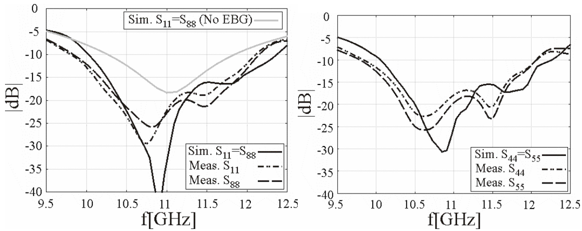
Figure 7: Measured and calculated input S-parameters for the 1D array prototype. The simulated S_{11} parameter of the same array without PCS-EBG is also shown.
