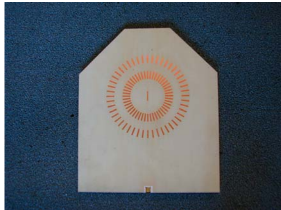
Figure 4: Panel portion containing the antenna surrounded by a PCS-EBG
