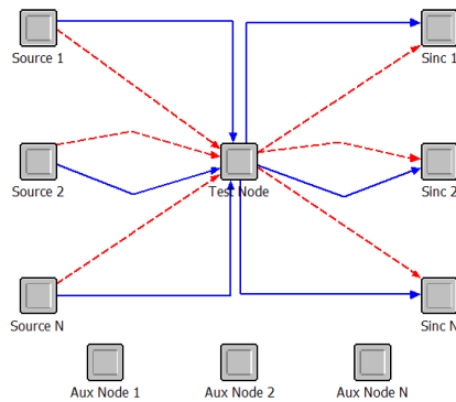
Figure 4.16: OPNET-Unit Conceptual Node Model. This node model serves as a communication tool to convey the intent of the actual node model in use by the framework, figure 4.17
