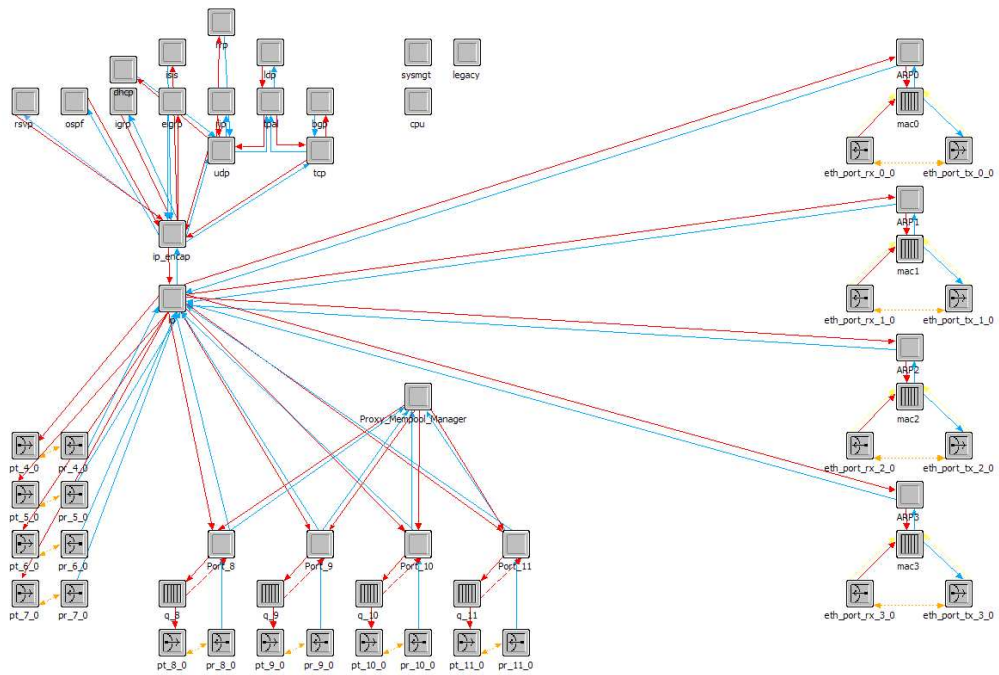
Figure 4.12: Strategy 2's Original Proxy Node Model. This node model is identical to strategy 1's Proxy node model (Figure 4.4), with the exception of the addition of the queuing process between the transceiver and the port process.
