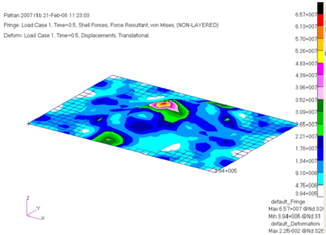
Figure 10. Stress distribution across a high-strength graphite epoxy plate, homogeneous.
