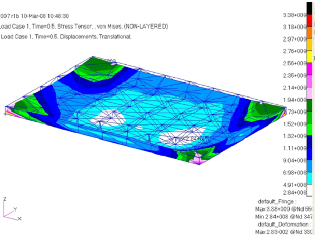
Figure 49. Maximum von Mises stress on a 3d steel plate at t = 0.5 sec.
