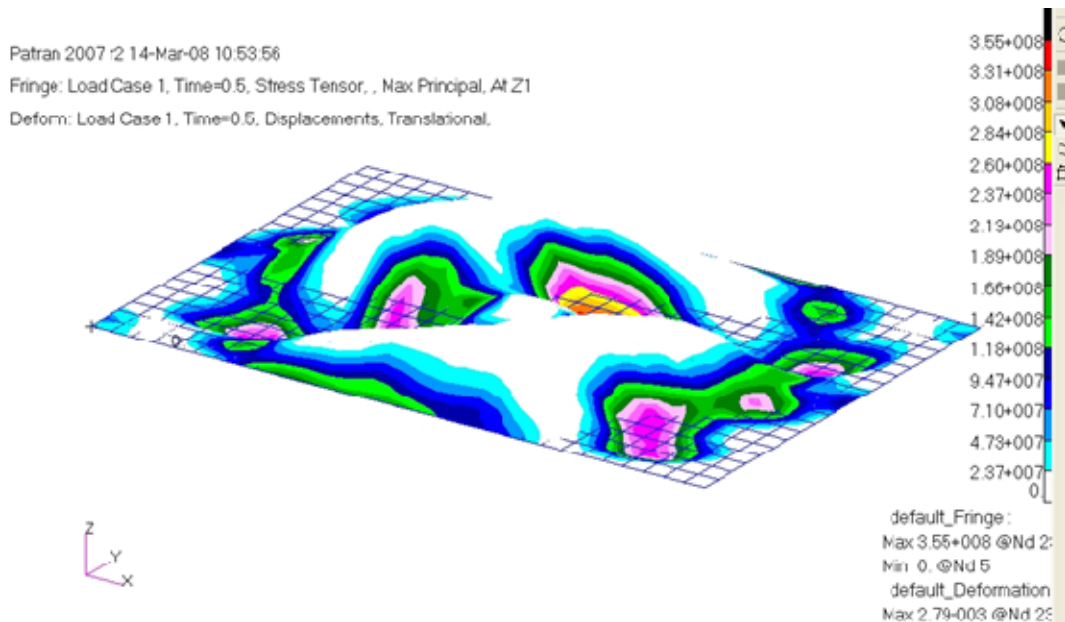
Figure 30. Tsai-Wu criteria stresses in high-modulus graphite.
