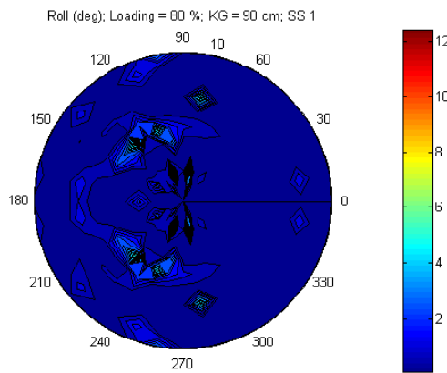
Figure 44. Roll at 80% Load, Sea State 1, Midbox Load.
