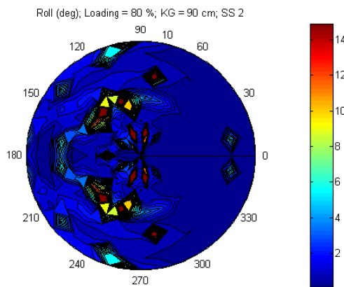
Figure 45. Roll at 80% Load, Sea State 2, Midbox Load.
