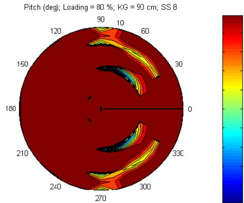
Figure 43. Pitch at 80% Load, Sea State 8, Midbox Load.
