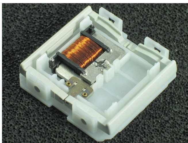
Figure 4: Energy converter of the switch module PTM 200. The magnetic circuit is operated via a lever-spring system (Product-Status)
