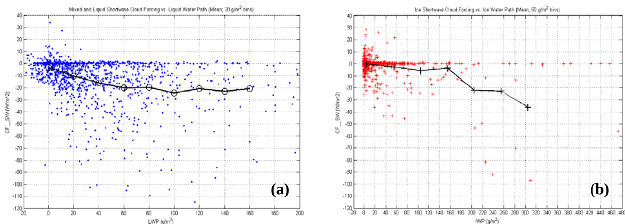
Figure 15. CF_SW for “liquid-containing” and ice-phase clouds in relation to LWP and IWP. CF_SW depends on available insolation. The greater the insolation, the greater the SW shading effect. For a given LWP (a) and IWP (b), the SW shading effect is stronger in “liquid-containing” clouds.
