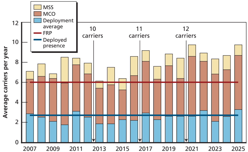
Figure 3.4 Current 32-Month Cycle Applied to the Fleet
