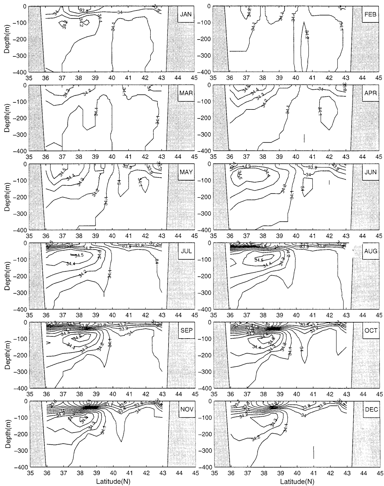
FIG. 15. Latitudinal cross section (135°E) of the monthly mean salinity. Contour interval: 0.1 psu.
