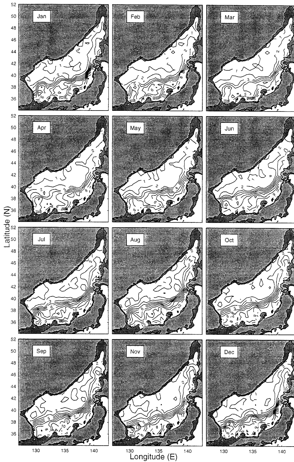
FIG. 6. Monthly mean temperature (°C) field at 150-m depth.
