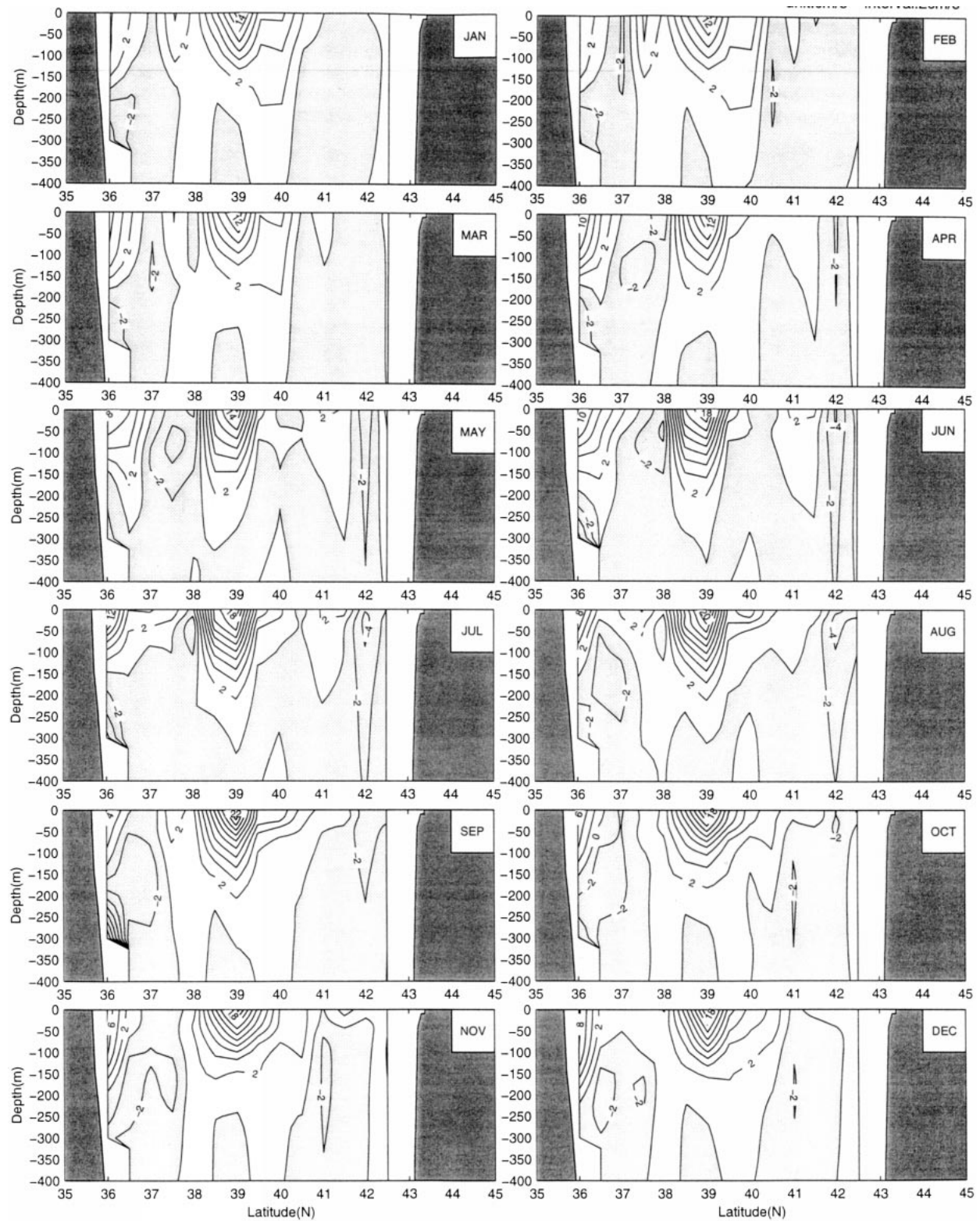
FIG. 17. Latitudinal cross sections of the inverted monthly mean u velocity along 135^{\circ}\text{E} . Contour interval: 2 \text{ cm s}^{-1} .
