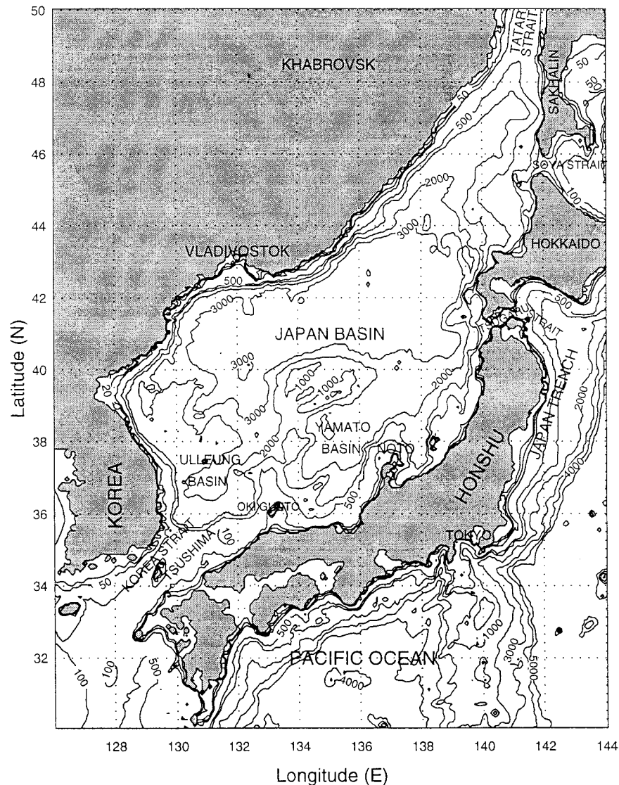
FIG. 1. Geography and isobaths showing the bottom topography (in meters) of the Japan/East Sea (JES).
