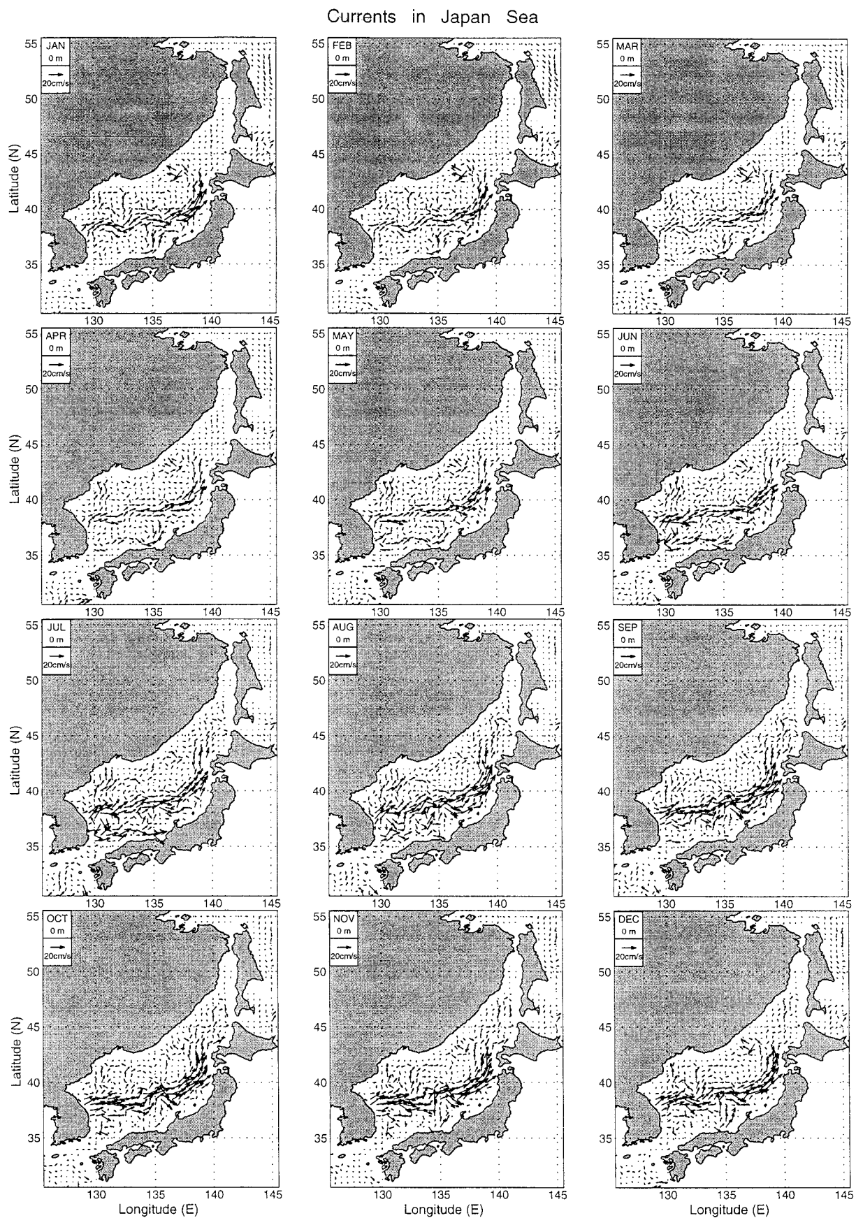
FIG. 16. Inverted monthly mean surface circulation.
