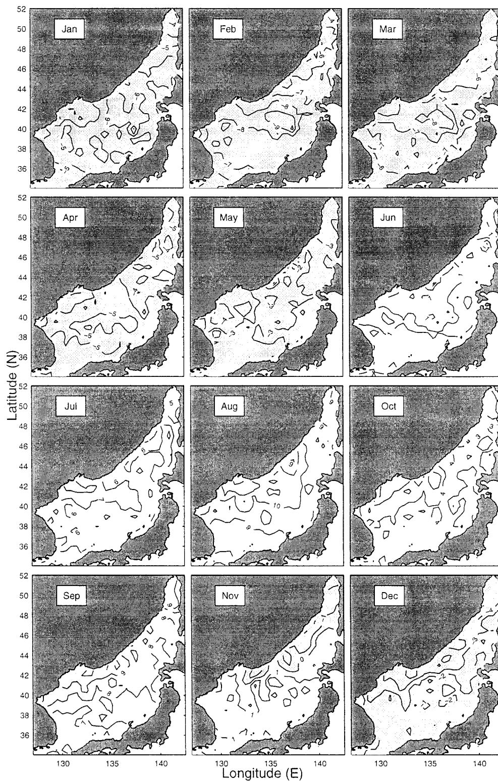
FIG. 5. Monthly mean temperature anomaly ( ^{\circ}\text{C} ) field at the ocean surface. Negative values are shaded.
