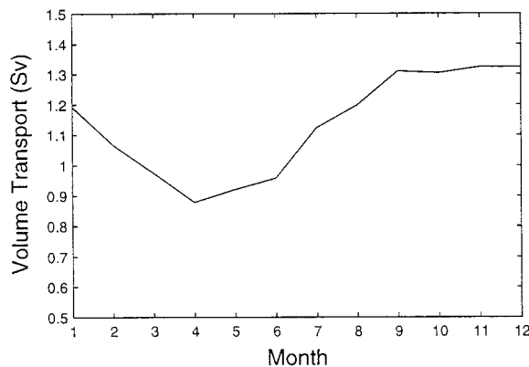
FIG. 18. Monthly variation of the volume transport (Sv) of the Polar Front Current at 135°E cross section.
