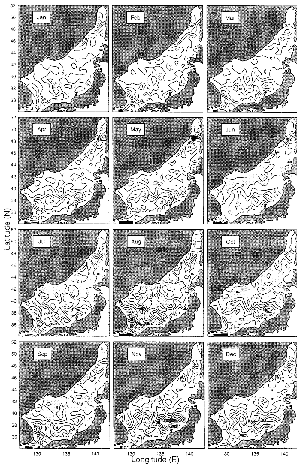
FIG. 11. Monthly mean salinity anomaly (psu) field at the ocean surface. Negative values are shaded.
