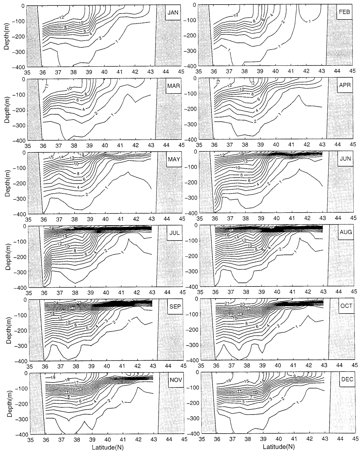
FIG. 9. Latitudinal cross section (135°E) of the monthly mean temperature (°C). Contour interval: 1°C.
