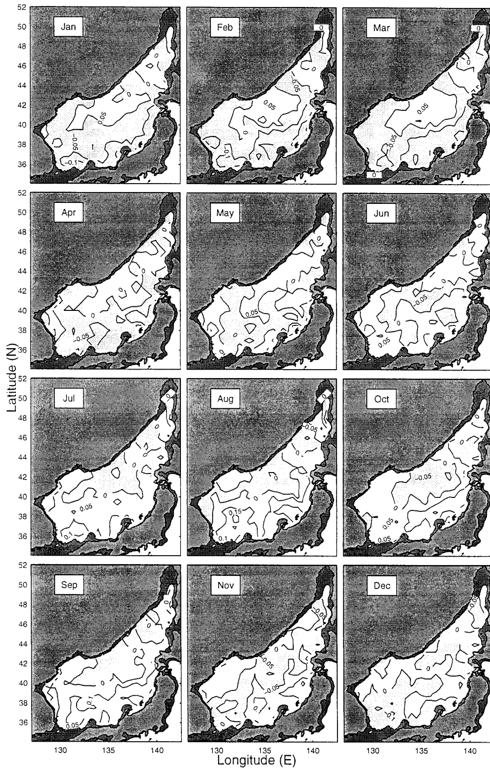
FIG. 13. Monthly mean salinity anomaly (psu) field at 150-m depth. Negative values are shaded.
