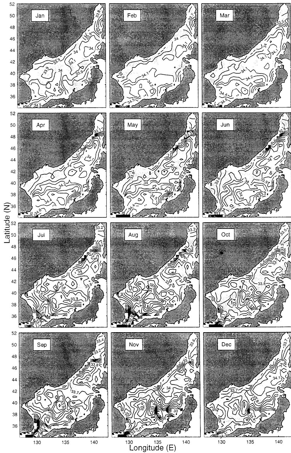
FIG. 10. Monthly mean salinity (psu) field at the ocean surface. Low salinity values ( S < 34.06 psu) are shaded.
