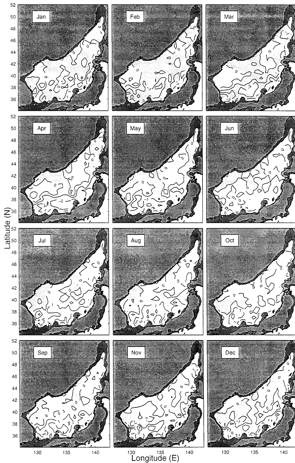
FIG. 7. Monthly mean temperature anomaly ( ^{\circ}\text{C} ) field at 150-m depth. Negative values are shaded.
