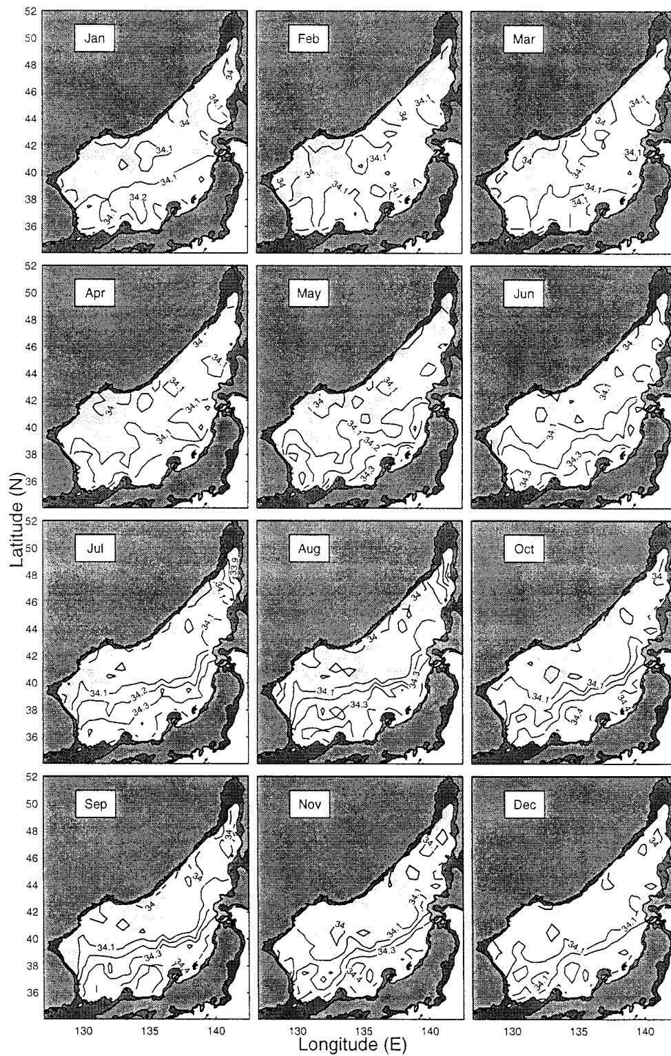
FIG. 12. Monthly mean salinity (psu) field at 150-m depth. Low salinity values ( S < 34.06 psu) are shaded.
