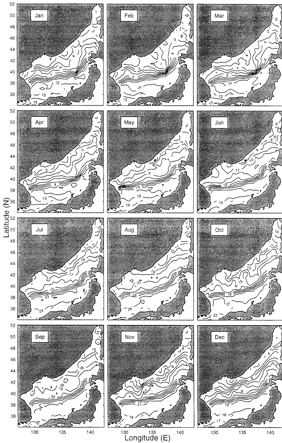
FIG. 4. Monthly mean temperature (°C) field at the ocean surface.
