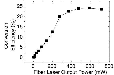
Figure 5: Total OPG Conversion Efficiency.
