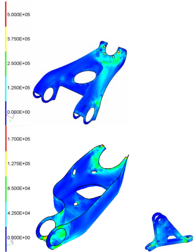
Figure 12. Overall Von Mises Stresses at 20,000 Cycles (a) Upper Control Arm, and (b) Lower Control Arm and Spring Support
