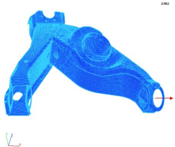
Figure 3. Finite Element Model of Control Arm with Load Direction for Load Case # 1
