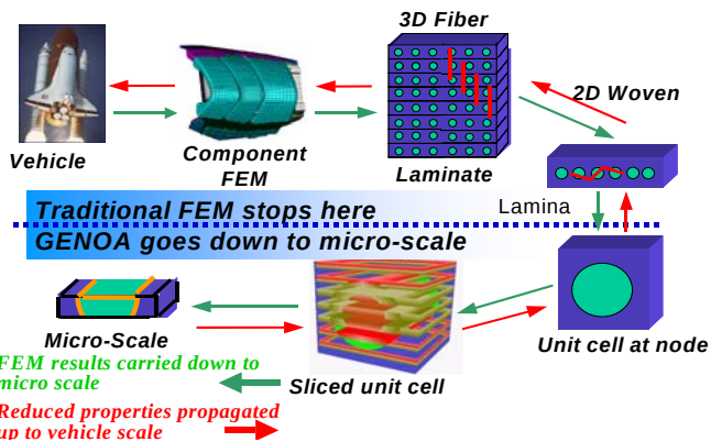
Figure 2. Hierarchical distribution of damage, stress, and strain from the macro to micro mechanical level.
