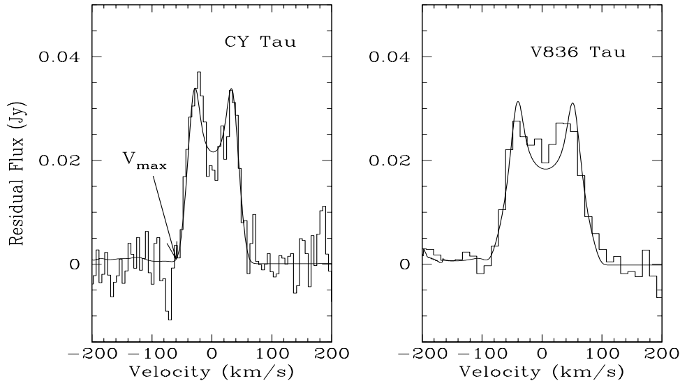
Figure 1. CO v = 1 - 0 line profiles for two CTTS that show a classic double-peaked disk profile (Najita, Carr & Mathieu 2003; Najita et al. 2007, in prep.). The smooth lines are model disk profiles. By measuring the maximum CO velocity in the profile, and knowing the stellar mass and inclination, the minimum CO gas radius follows for Keplerian rotation.
