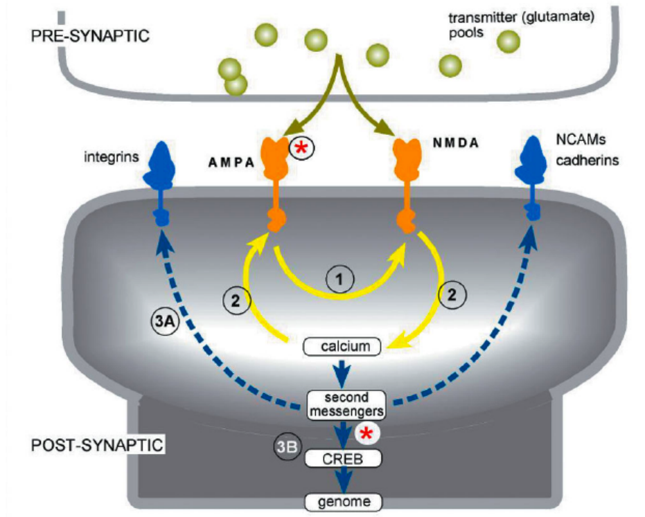
Figure 3.6: Interconnected biochemical cycles. Ampakine-induced increase in AMPA activity directly affects NMDA response in admitting calcium ions. Increased \text{Ca}^{2+} concentration increase subsequent AMPA response (path 2), and cause long-term changes in the effectiveness and number of AMPA receptors (paths 3A and 3B). Path 3A involves changes in the cytoplasmic region near AMPA. Path 3b involves gene-signaling pathways including the CREB transcription factors. Figure from reference [36].
