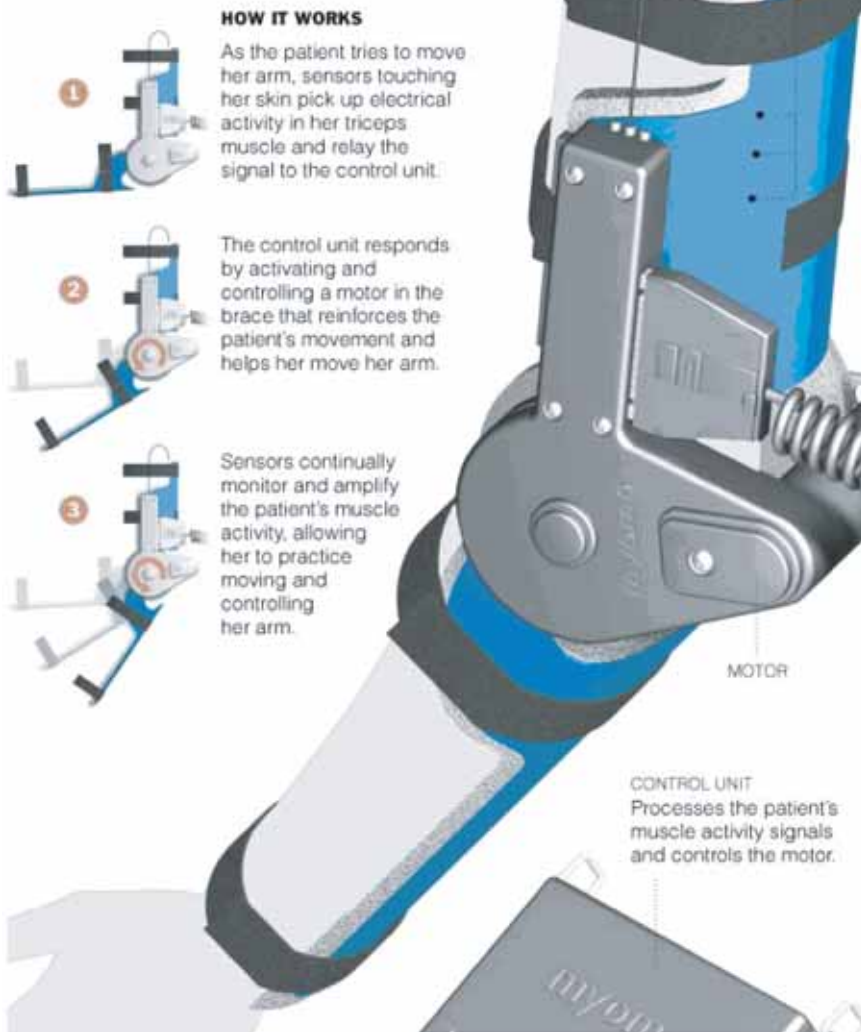
Figure 3.4: The Myomo e100 robotic device senses weak electrical activity in a patients arm muscles and uses this signal to actuate a mechanical unit to move the lower arm as shown in the diagram at left. This assist allows patients to retrain their own muscle control system to regain a measure of use of the arm to do tasks they had been unable to do after the stroke. After New York Times (July 10, 2007).
