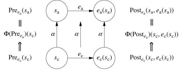
Fig. 2. Relations to establish between concrete and abstract transitions and preconditions and postconditions.
