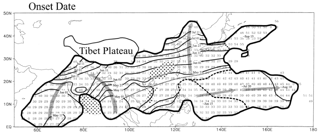
Figure 1. Average dates at which Asian summer monsoon precipitation begins, shown by dates along thin black contour lines (from Wang and Linho 2002).
