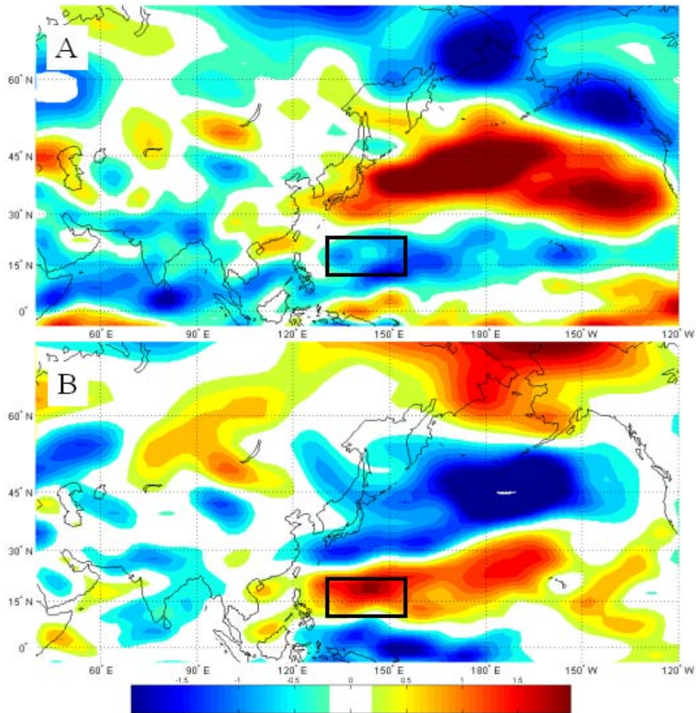
Figure 30. (A) HP and (B) LP composites of anomalous 925 hPa zonal wind in April prior to the KSM. Units are meters per second.
