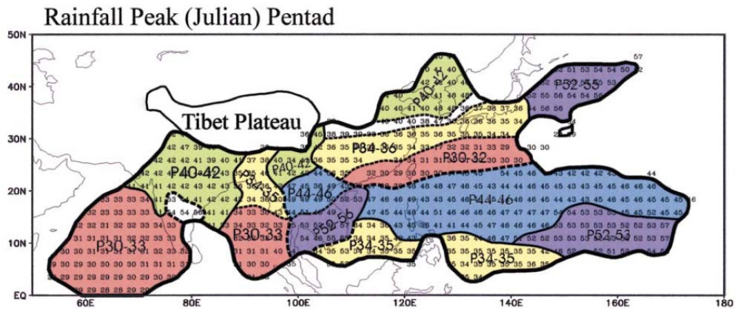
Figure 2. Peak precipitation by pentad (P30 - P55) for each major subsystem of the Asian summer monsoon (shown by colored regions) (from Wang and Linho 2002).
