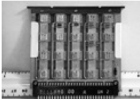
Figure 8. UYK 7 printed circuit board 30 (From McHale)
