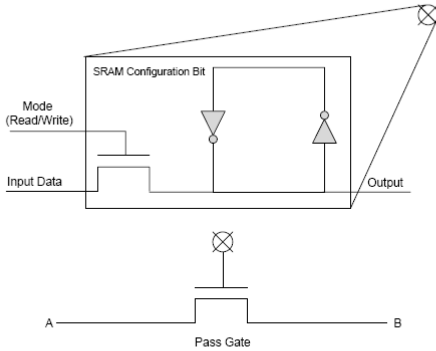
Figure 5. Generic routing architecture 19 (From Barzargan)
