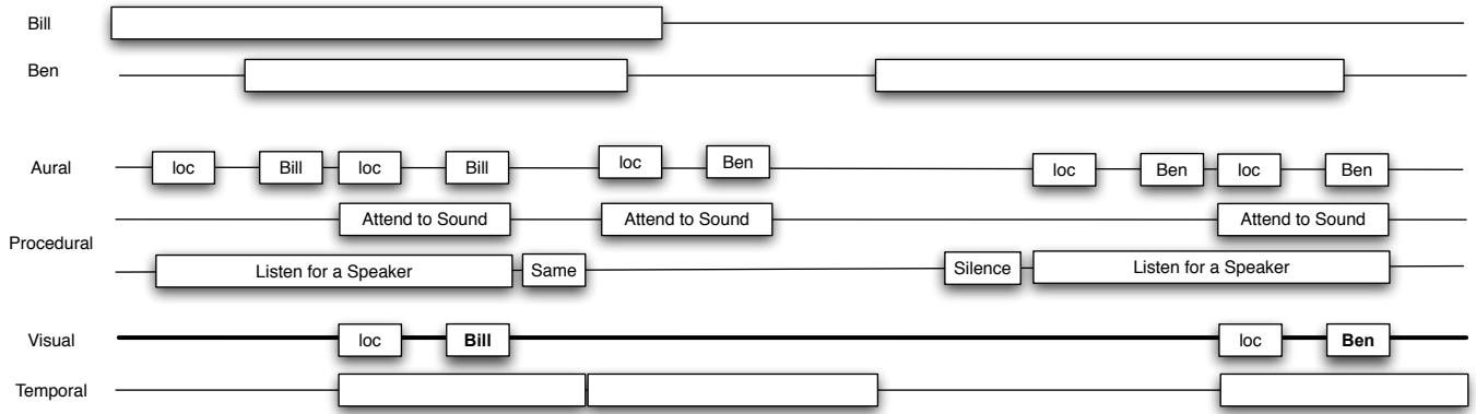
Figure 5: Time-Graph of a sample run of the conversation tracking model.
