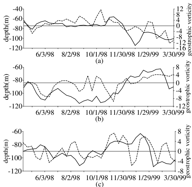
Figure 4. Time series of 22°C isotherm depth (solid line) and geostrophic vorticity (dashed line) at (a) SCS1; (b) SCS2; (c) SCS3.
