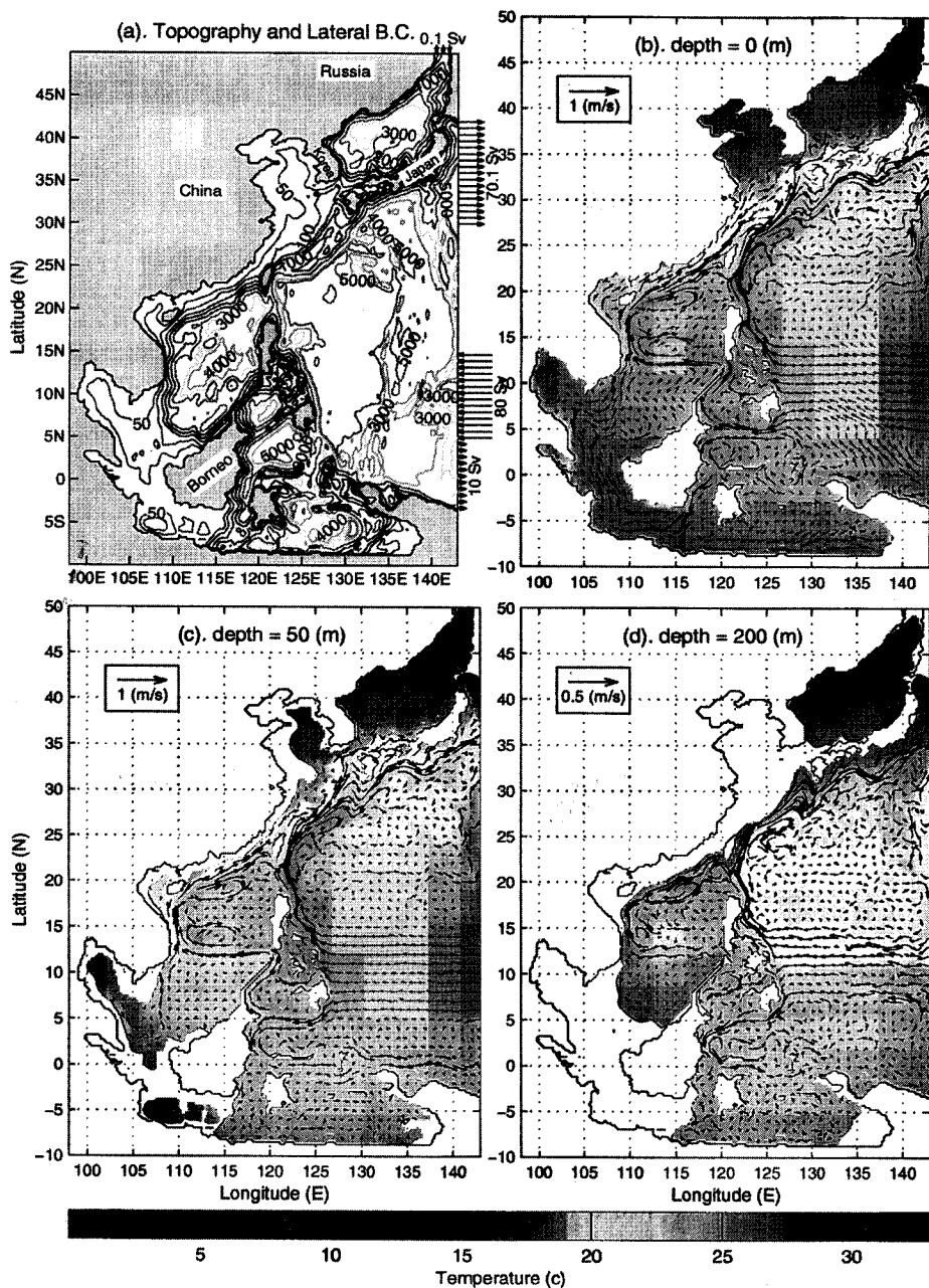
Fig. 1. Predicted temperature and velocity fields in June 1998
