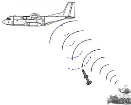
Figure 5. Semi-active guidance.
