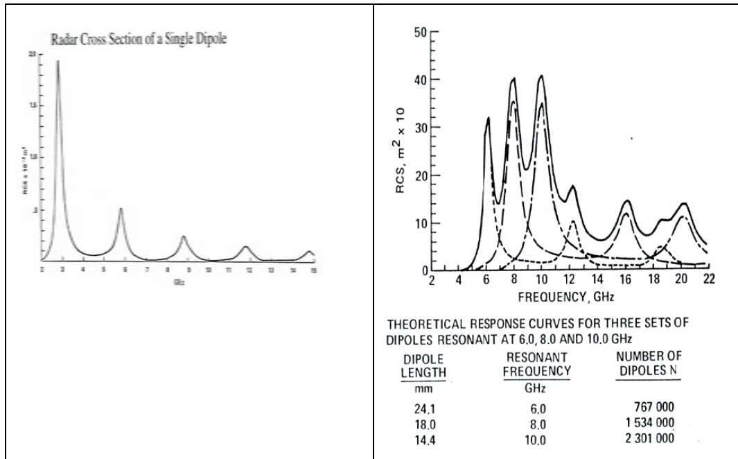
Figure 49. Backscatter from a single dipole and three dipoles. 51
