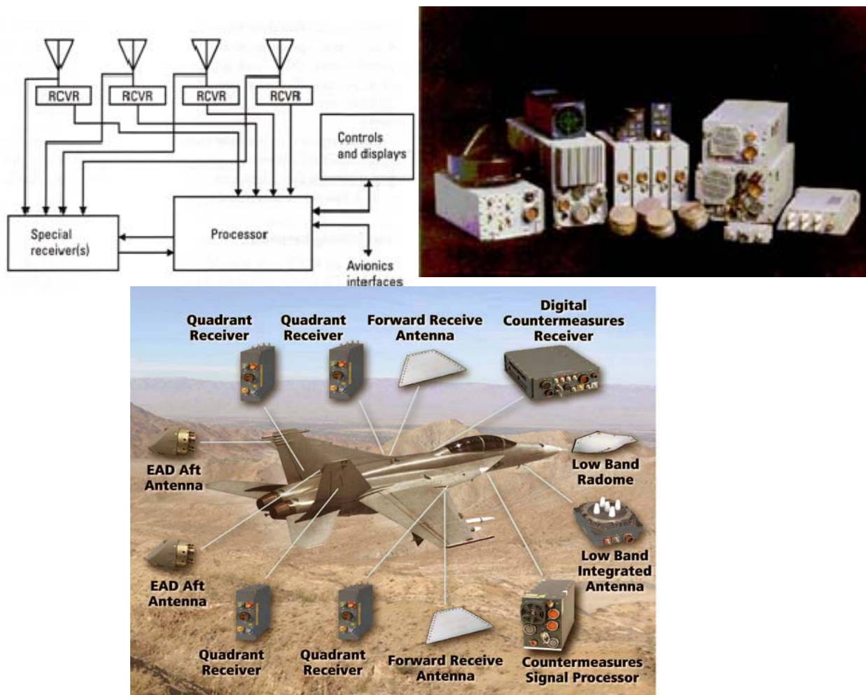
Figure 40. RWR System Components. 36
