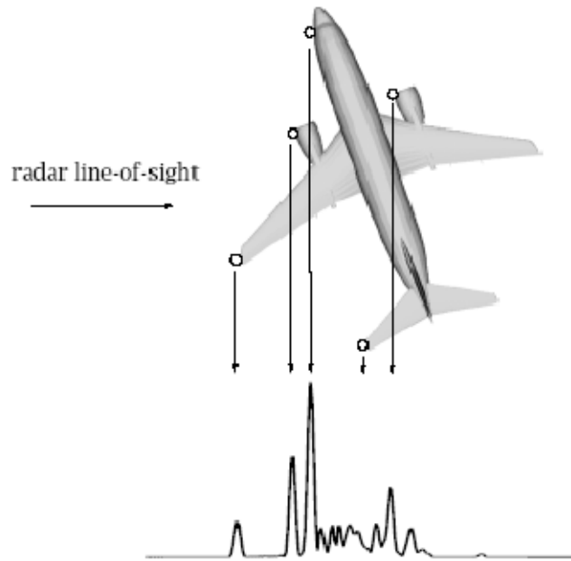
Figure 26. Example of a range profile of Boeing 737-500. 25
