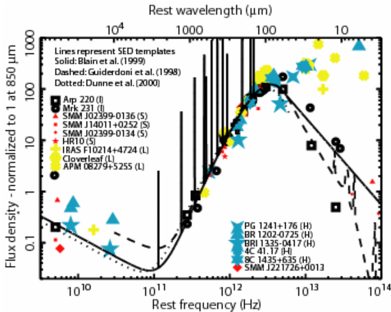
Figure 4 –The far-IR spectrum of a galaxy 40 contains a large fraction of the bolometric luminosity and many strong emission lines, which can be used to calculate physical conditions in the interstellar medium, estimate rates of star formation, and measure a galaxy’s redshift. SPIRIT will be able to measure the line intensities and the far-IR spectral energy distributions of galaxies out to high redshifts to probe the epoch of most-intense star formation ( z \sim 2 - 3 ), distinguish between nuclear and non-nuclear emission, and determine the relationship between galaxy mergers and star formation activity.
