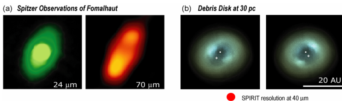
Figure 2 – Spitzer resolves four nearby debris disks, including Fomalhaut, shown here (a) at 24 and 70 \mu\text{m} . 27 With angular resolution a hundred-fold better than that of Spitzer, SPIRIT will provide clear images of a large statistical sample of debris disks, enabling discoveries of new planets and a great improvement in our understanding of the factors that influence the evolution of planetary systems. The model images in (b), based on Eps Eri but scaled to 30 pc, show the predicted far-IR emission at 40 , 60 , and 100 \mu\text{m} color-coded as blue, green, and red, respectively. The dust-trapping planet (+) is shown at two orbital phases, and the resonantly trapped dust grains can be seen to have moved.
