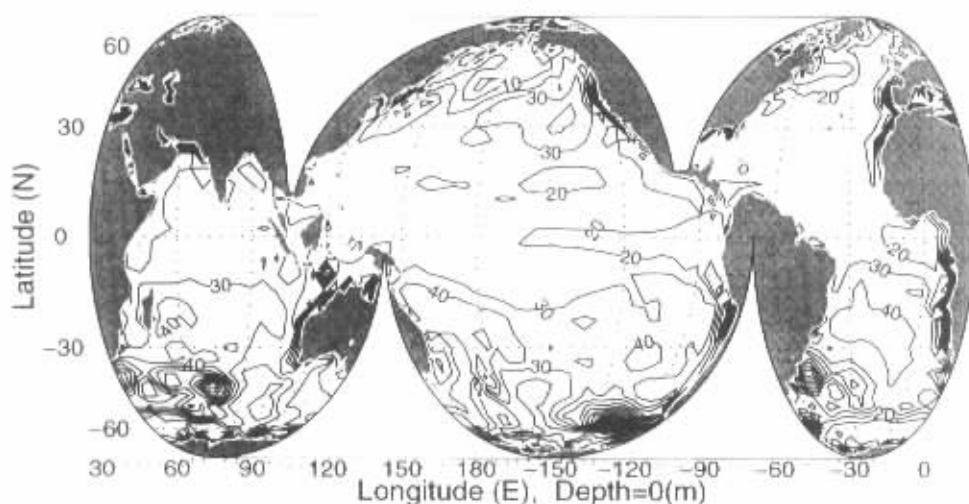
Fig. 5. Monthly mean surface sensible heat flux ( W/m^2 ) simulated by the GISS Coupled Model. (a) January 1978, and (b) July 1978.
