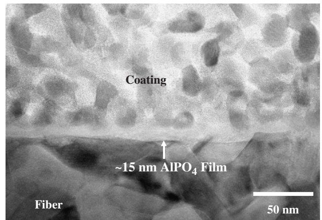
Fig. 6. Transmission electron micrograph of as-deposited (Y,La)PO 4 fiber coatings on Nextel 720, showing a thin film of AlPO 4 in the coating fiber interphase.
