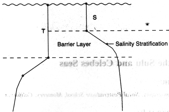
FIG. 1. A diagram of isothermal, mixed, and barrier layers.
