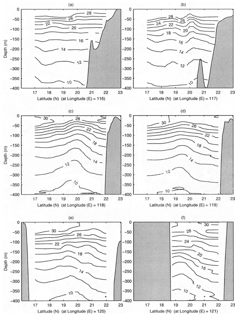
Fig. 8. Temperature distribution at several latitudinal cross sections: (a) 116°E, (b) 117°E, (c) 118°E, (d) 119°E, (e) 120°E, and (f) 121°E.
