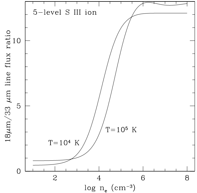
FIG. 9.—The 18\ \mu\text{m}/33\ \mu\text{m} line flux ratio in \text{S III} vs. electron density n_e , for gas temperatures T = 10^4 and 10^5\ \text{K} .
