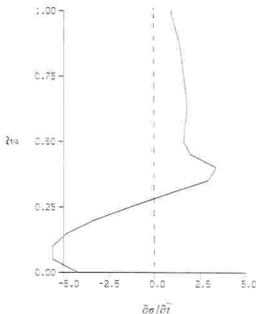
Fig. 4. Vertical dependency of \partial\sigma/\partial\tilde{t} for the vortex with Bu=1 , Ro=0.1 , m_i=4 , and m_e=4 .
