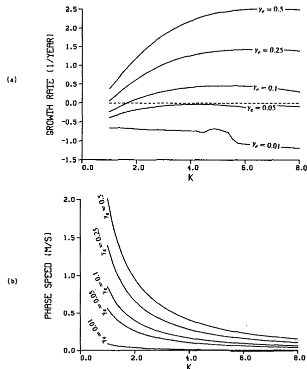
FIG. 8. Dependence of the low-frequency AOSHE S-Mode on the entrainment parameter \gamma_e : (a) growth rate and (b) phase speed. The other important parameters are \gamma^{(s)} = 0.01 , \alpha_s^{(s)} = 0.006 , F = 0.1 , \epsilon_p = 0.8 , and \lambda = 1 .
