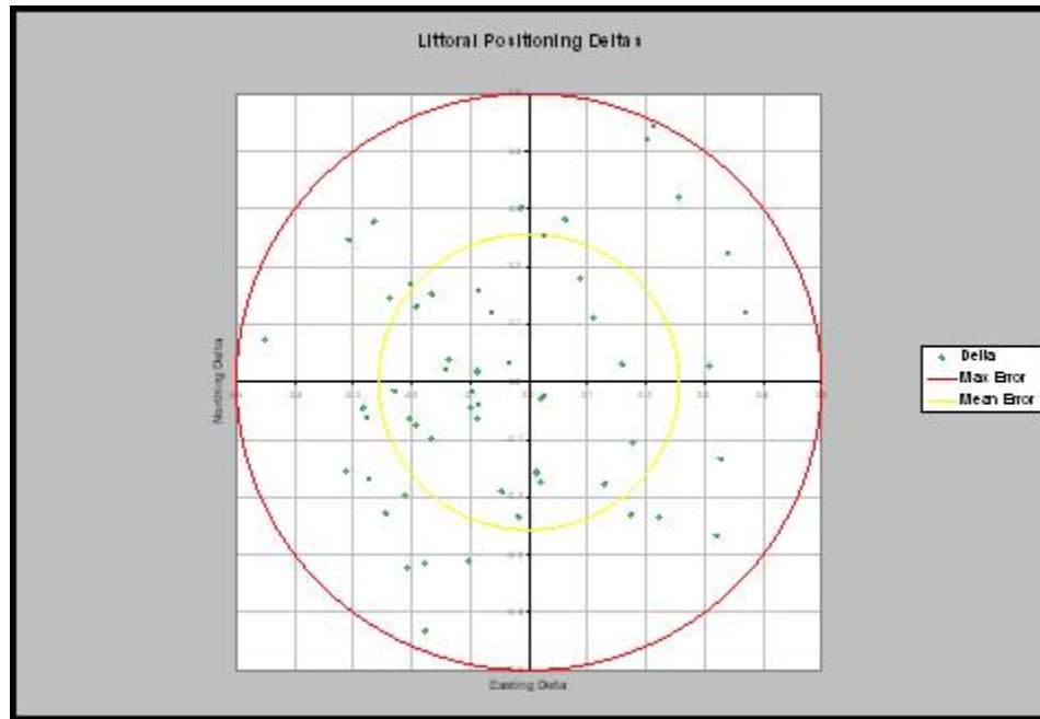
Figure 16. Littoral positioning error scatter-graph.
