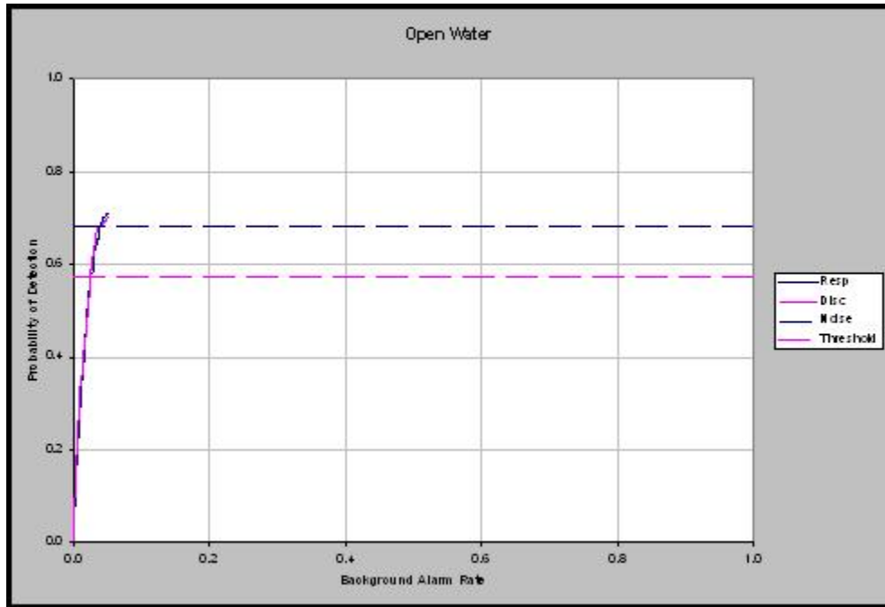
Figure 11. Open water P_d versus BAR.
