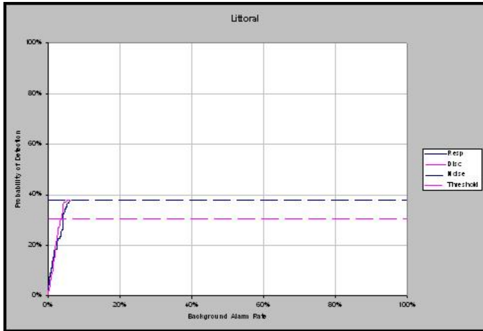
Figure 13. Littoral P_d versus BAR.
