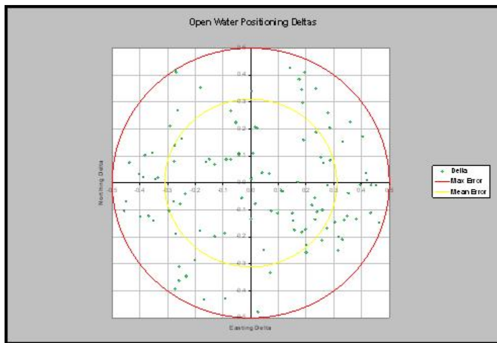
Figure 15. Open water positioning error scatter-graph.
