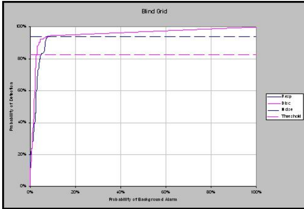
Figure 9. Blind grid P_d versus P_{ba} .
