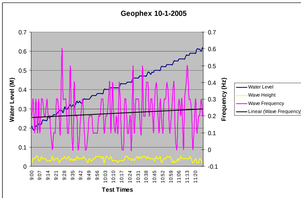
Figure A-4. Water conditions on 1 October 2005.
