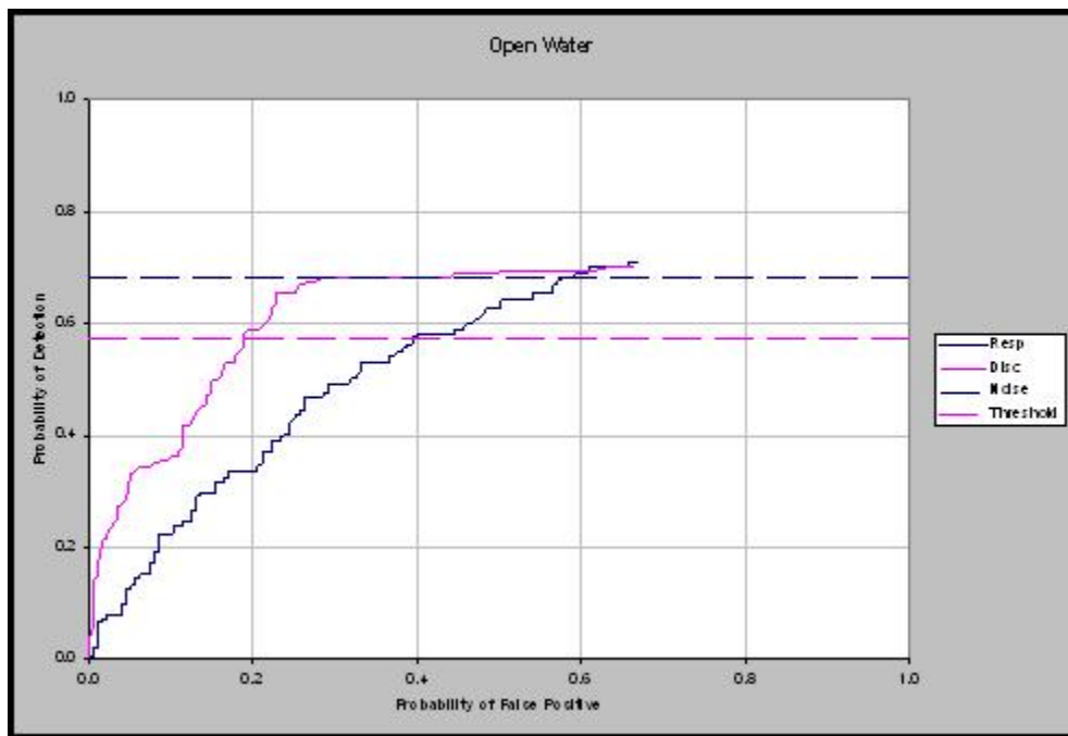
Figure 10. Open water P_d versus P_{fp} .
