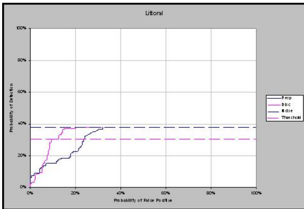
Figure 12. Littoral P_d versus P_{fp} .
