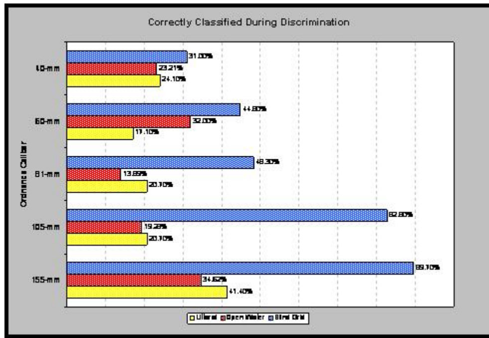
Figure 14. Percent of ordnance correctly classified during the discrimination stage.
