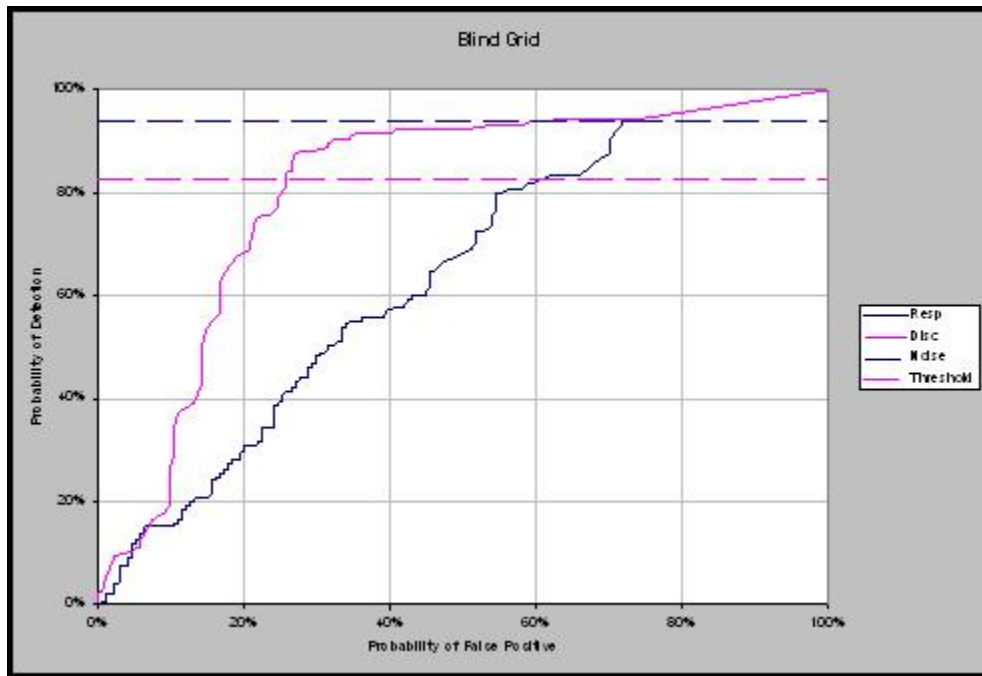
Figure 8. Blind grid P_d versus P_{fp} .
