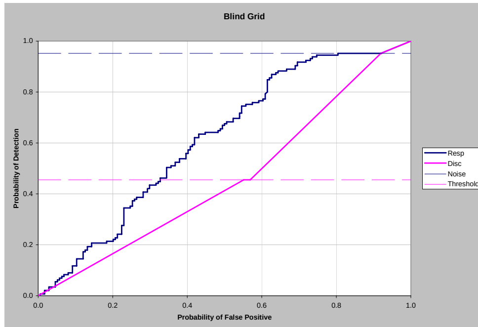
Figure 9. Blind grid P_d versus P_{fp} .
