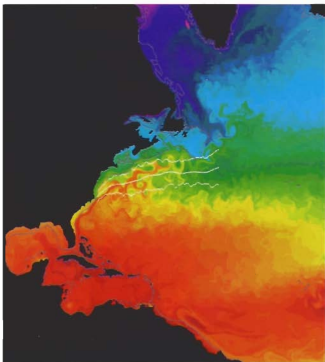
Figure 2: Sea Surface Temperature (SST) field from the fine-mesh simulation at day 273, year 14, performed with the Miami Isopycnal Coordinate Ocean Model (MICOM). Red denotes warm temperatures, blue cold temperatures. The observed mean position of the Gulf Stream is represented by the center line. The envelope is defined by the outer lines.
